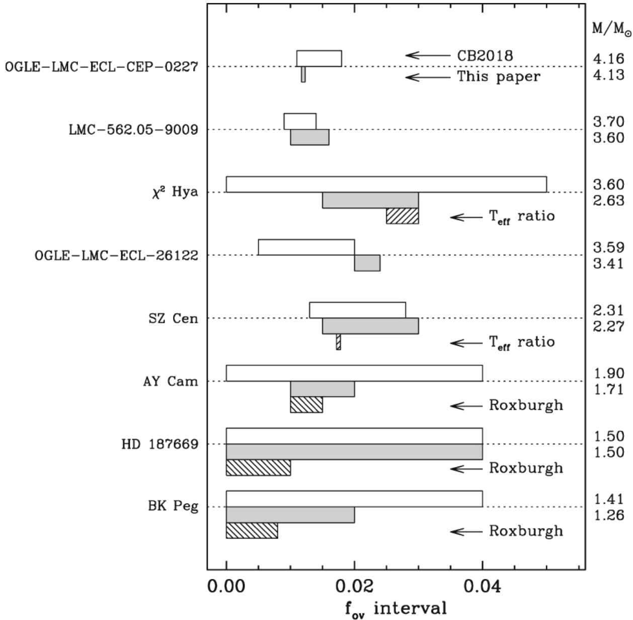
Figure 9. from The Dependence of Convective Core Overshooting on Stellar Mass: Reality Check and Additional Evidence null 2019 APJ 876 134 doi:10.3847/1538-4357/ab1589 https://dx.doi.org/10.3847/1538-4357/ab1589 © 2019. The American Astronomical Society. All rights reserved.
