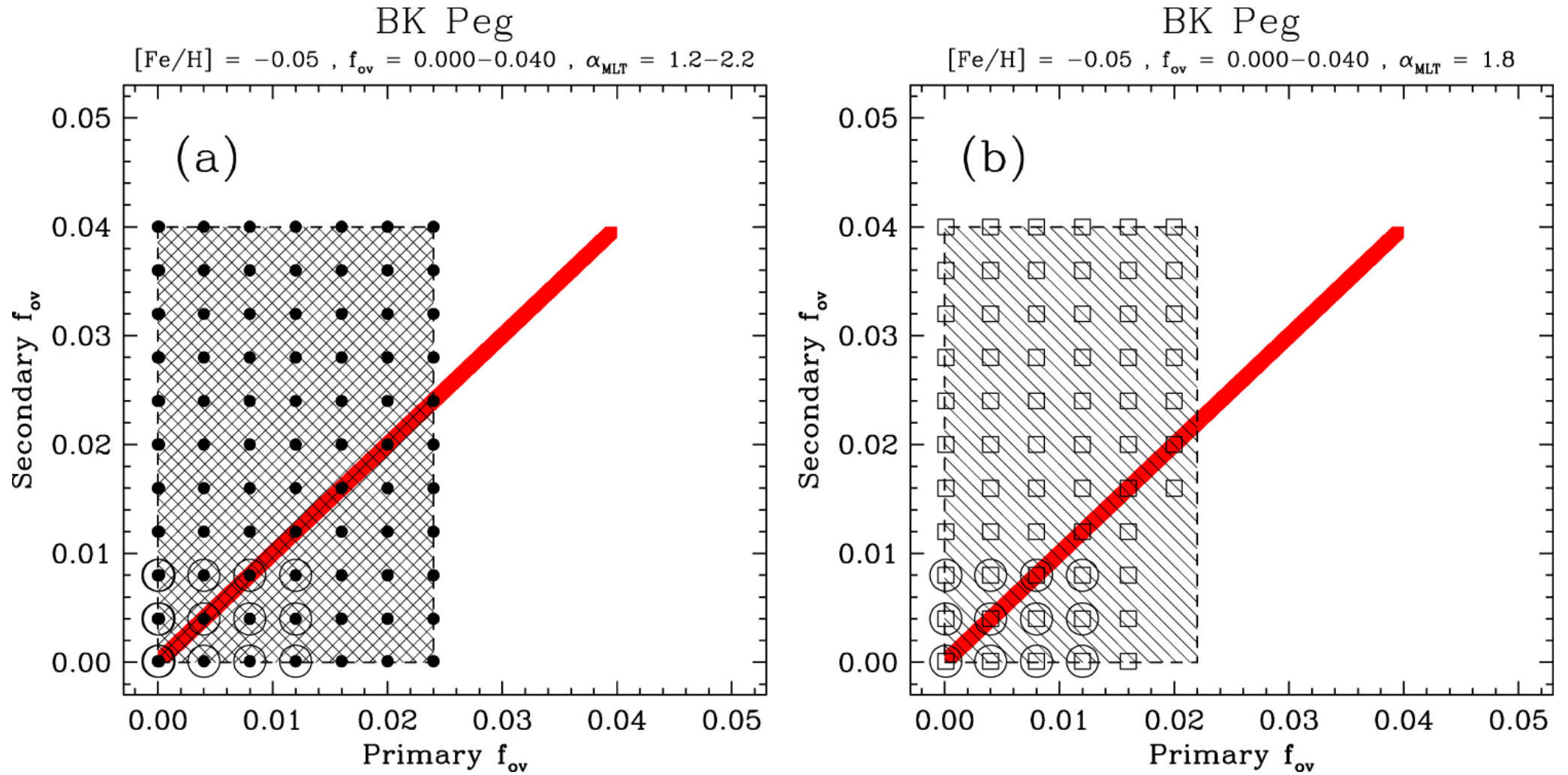
Figure 8. from The Dependence of Convective Core Overshooting on Stellar Mass: Reality Check and Additional Evidence null 2019 APJ 876 134 doi:10.3847/1538-4357/ab1589 https://dx.doi.org/10.3847/1538-4357/ab1589 © 2019. The American Astronomical Society. All rights reserved.
