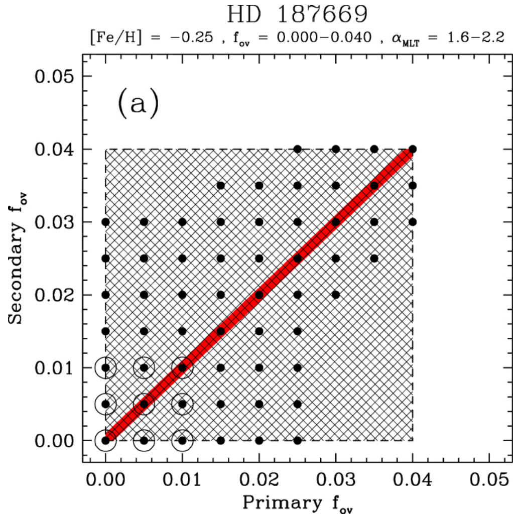
Figure 7. from The Dependence of Convective Core Overshooting on Stellar Mass: Reality Check and Additional Evidence null 2019 APJ 876 134 doi:10.3847/1538-4357/ab1589 https://dx.doi.org/10.3847/1538-4357/ab1589 © 2019. The American Astronomical Society. All rights reserved.
