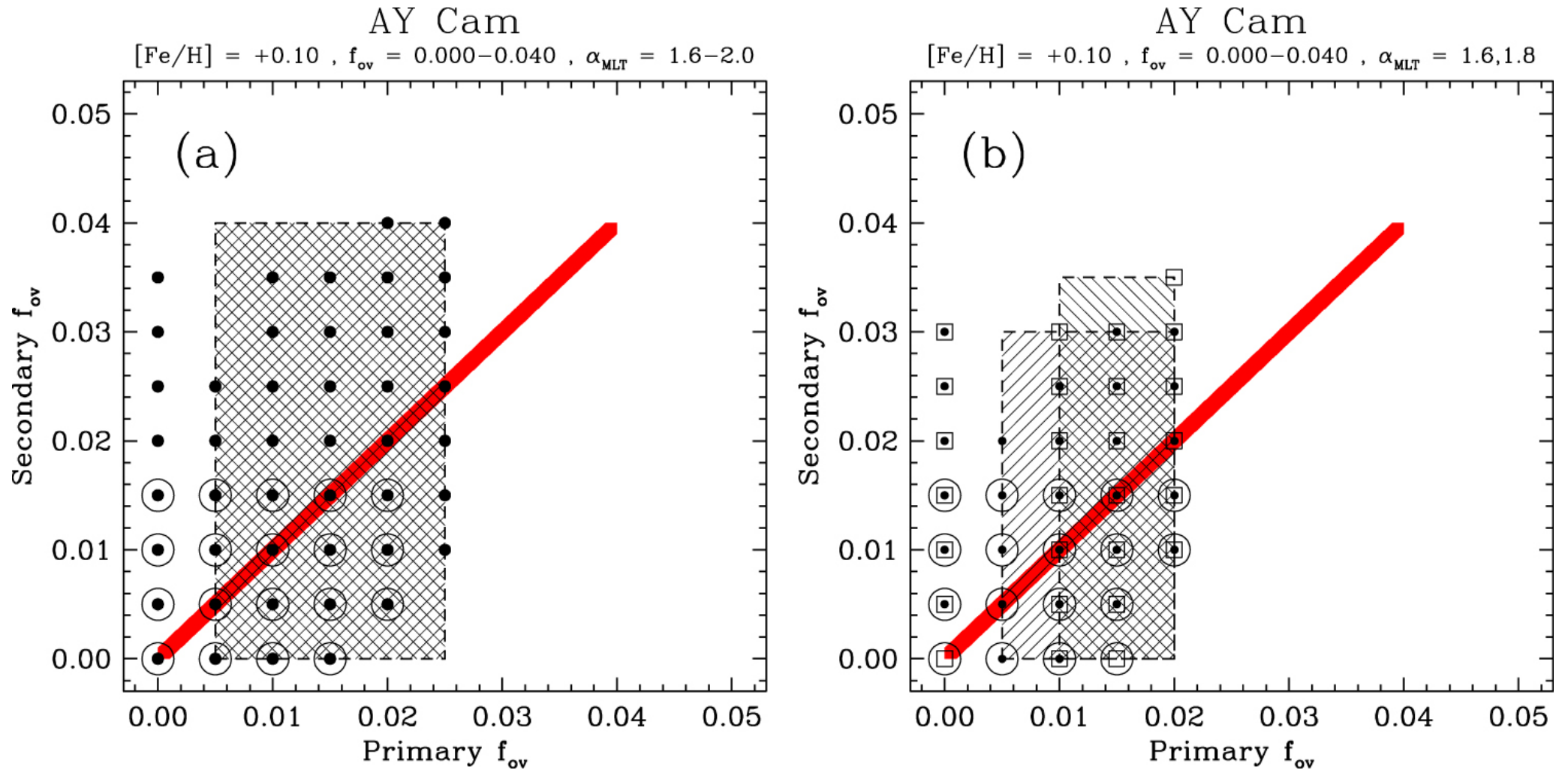
Figure 6. from The Dependence of Convective Core Overshooting on Stellar Mass: Reality Check and Additional Evidence null 2019 APJ 876 134 doi:10.3847/1538-4357/ab1589 https://dx.doi.org/10.3847/1538-4357/ab1589 © 2019. The American Astronomical Society. All rights reserved.
