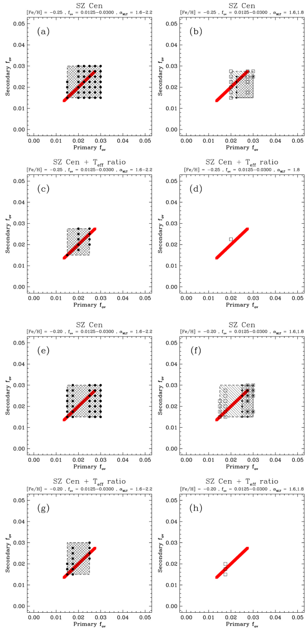
Figure 5. from The Dependence of Convective Core Overshooting on Stellar Mass: Reality Check and Additional Evidence null 2019 APJ 876 134 doi:10.3847/1538-4357/ab1589 https://dx.doi.org/10.3847/1538-4357/ab1589 © 2019. The American Astronomical Society. All rights reserved.
