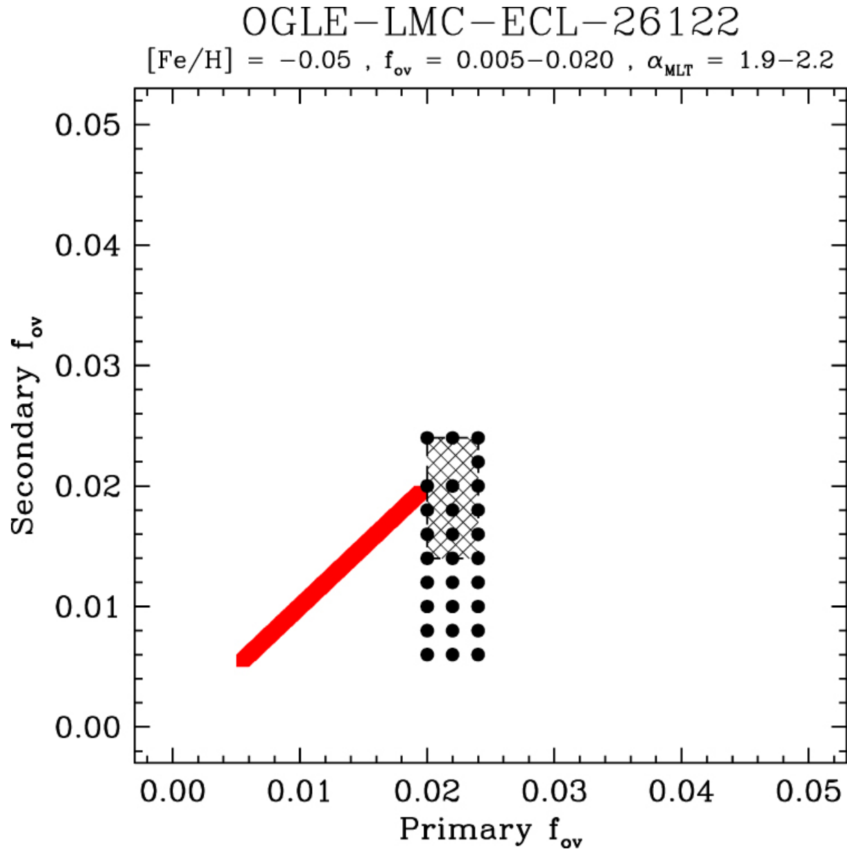
Figure 4. from The Dependence of Convective Core Overshooting on Stellar Mass: Reality Check and Additional Evidence null 2019 APJ 876 134 doi:10.3847/1538-4357/ab1589 https://dx.doi.org/10.3847/1538-4357/ab1589 © 2019. The American Astronomical Society. All rights reserved.
