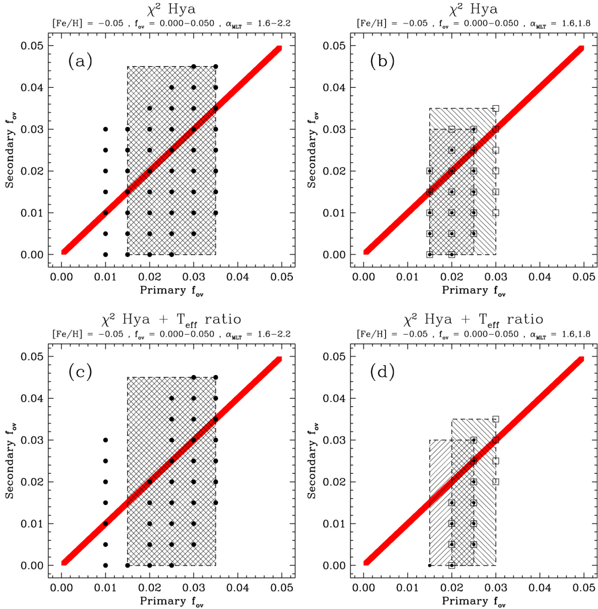
Figure 3. from The Dependence of Convective Core Overshooting on Stellar Mass: Reality Check and Additional Evidence null 2019 APJ 876 134 doi:10.3847/1538-4357/ab1589 https://dx.doi.org/10.3847/1538-4357/ab1589 © 2019. The American Astronomical Society. All rights reserved.
