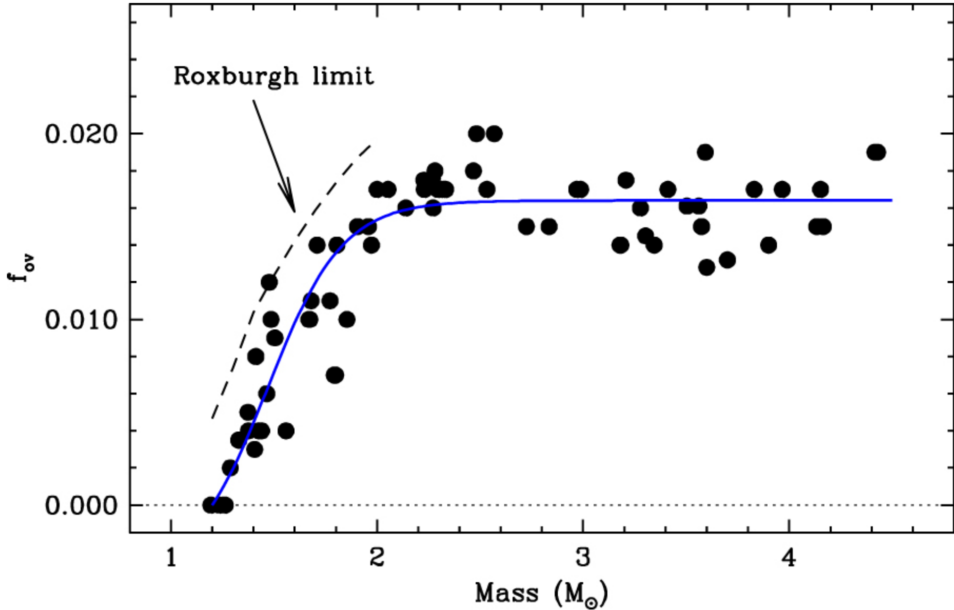
Figure 13. from The Dependence of Convective Core Overshooting on Stellar Mass: Reality Check and Additional Evidence null 2019 APJ 876 134 doi:10.3847/1538-4357/ab1589 https://dx.doi.org/10.3847/1538-4357/ab1589 © 2019. The American Astronomical Society. All rights reserved.
