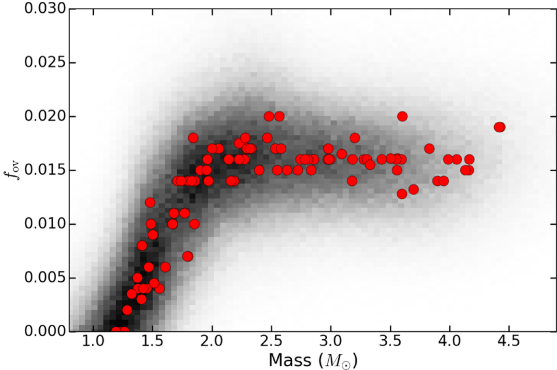
Figure 10. from The Dependence of Convective Core Overshooting on Stellar Mass: Reality Check and Additional Evidence null 2019 APJ 876 134 doi:10.3847/1538-4357/ab1589 https://dx.doi.org/10.3847/1538-4357/ab1589 © 2019. The American Astronomical Society. All rights reserved.
