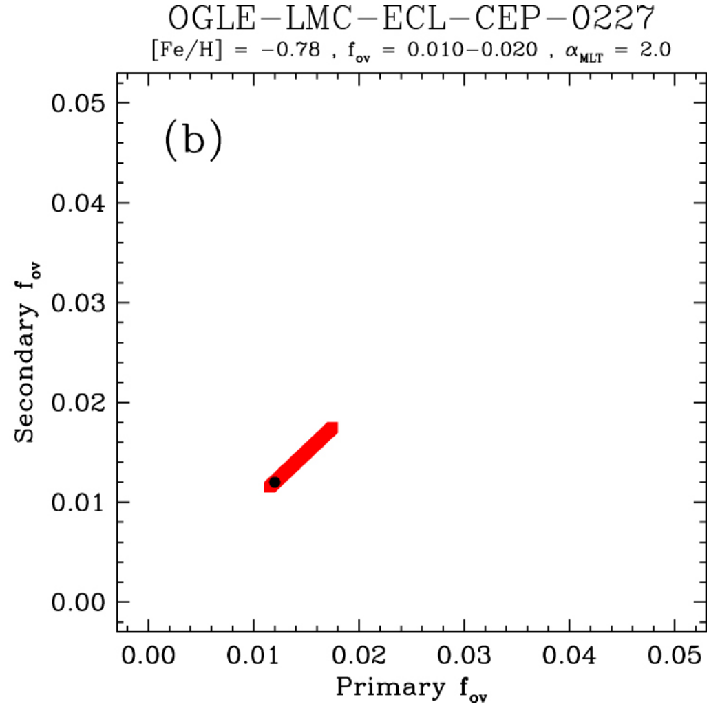
Figure 1. from The Dependence of Convective Core Overshooting on Stellar Mass: Reality Check and Additional Evidence null 2019 APJ 876 134 doi:10.3847/1538-4357/ab1589 https://dx.doi.org/10.3847/1538-4357/ab1589
