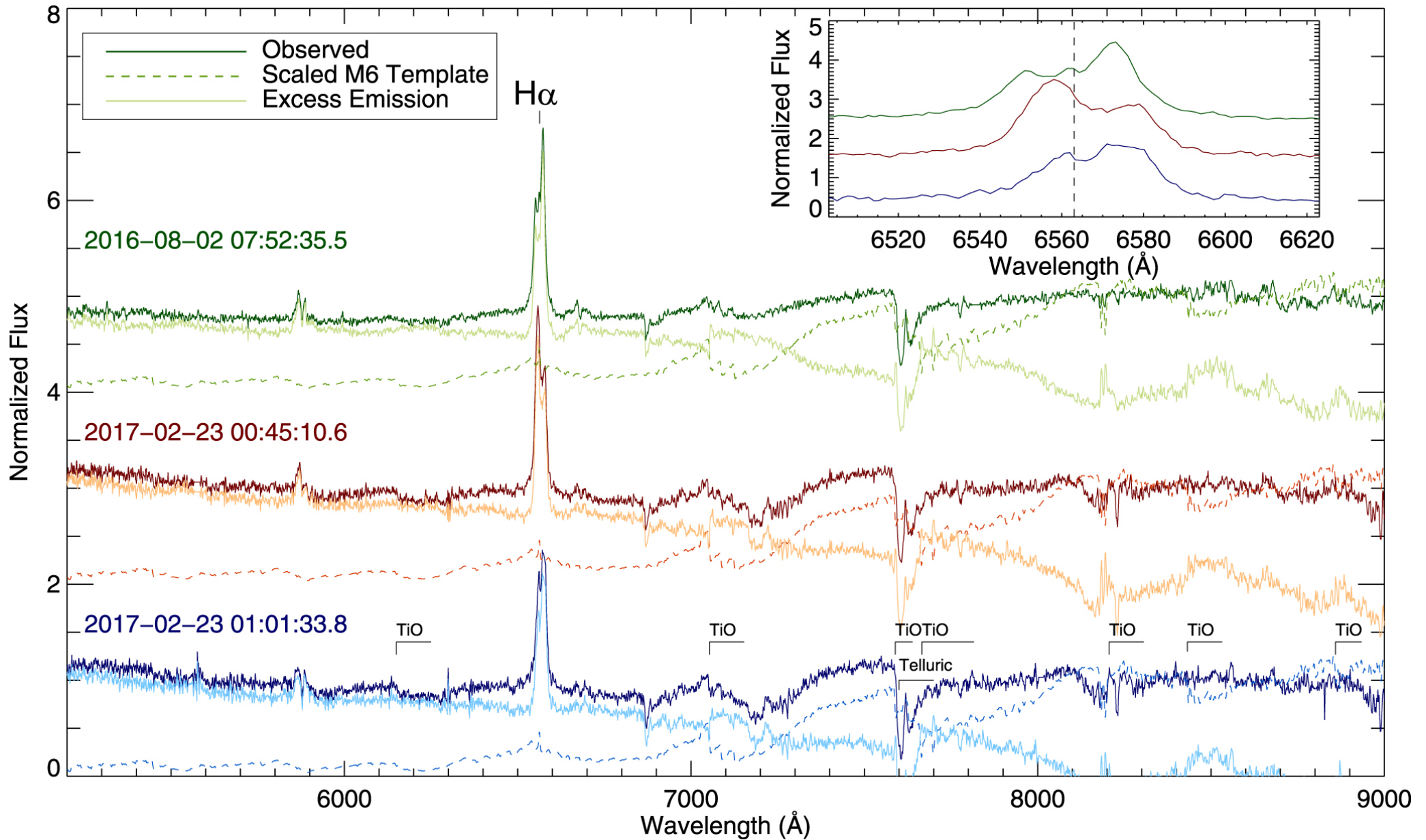
Figure 8. from The Largest M Dwarf Flares from ASAS-SN null 2019 APJ 876 115 doi:10.3847/1538-4357/ab148d https://dx.doi.org/10.3847/1538-4357/ab148d © 2019. The American Astronomical Society. All rights reserved.
