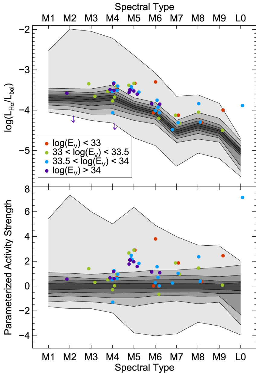
Figure 7. from The Largest M Dwarf Flares from ASAS-SN null 2019 APJ 876 115 doi:10.3847/1538-4357/ab148d https://dx.doi.org/10.3847/1538-4357/ab148d © 2019. The American Astronomical Society. All rights reserved.
