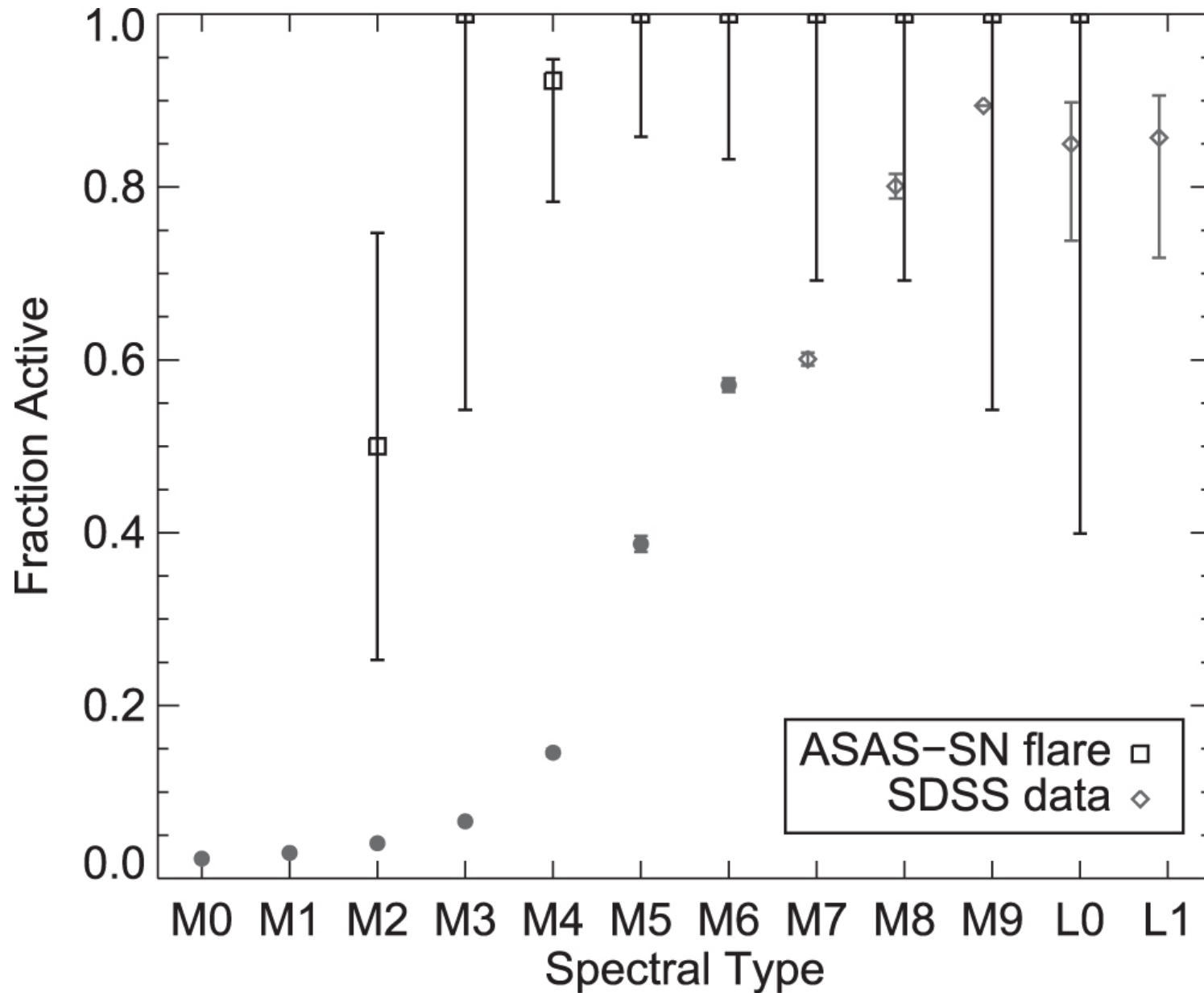
Figure 6. from The Largest M Dwarf Flares from ASAS-SN null 2019 APJ 876 115 doi:10.3847/1538-4357/ab148d https://dx.doi.org/10.3847/1538-4357/ab148d © 2019. The American Astronomical Society. All rights reserved.
