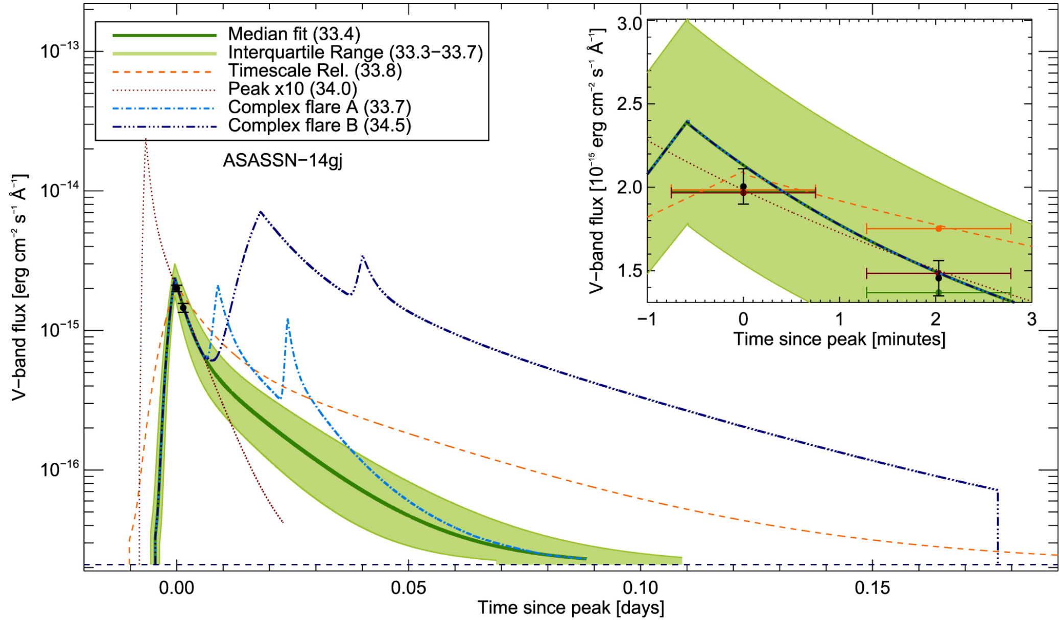
Figure 5. from The Largest M Dwarf Flares from ASAS-SN null 2019 APJ 876 115 doi:10.3847/1538-4357/ab148d https://dx.doi.org/10.3847/1538-4357/ab148d © 2019. The American Astronomical Society. All rights reserved.
