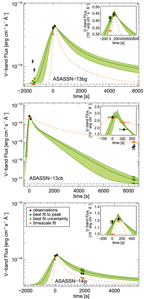
Figure 4. from The Largest M Dwarf Flares from ASAS-SN null 2019 APJ 876 115 doi:10.3847/1538-4357/ab148d https://dx.doi.org/10.3847/1538-4357/ab148d © 2019. The American Astronomical Society. All rights reserved.
