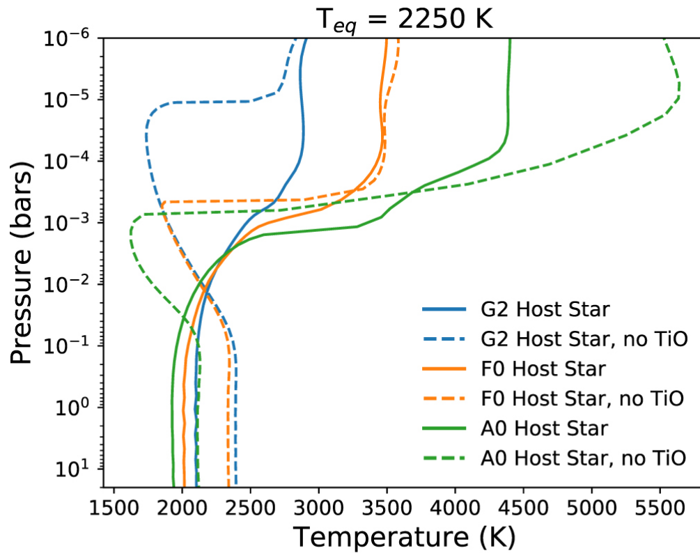
Figure 3. from The Influence of Host Star Spectral Type on Ultra-hot Jupiter Atmospheres null 2019 APJ 876 69 doi:10.3847/1538-4357/ab1485 https://dx.doi.org/10.3847/1538-4357/ab1485 © 2019. The American Astronomical Society. All rights reserved.
