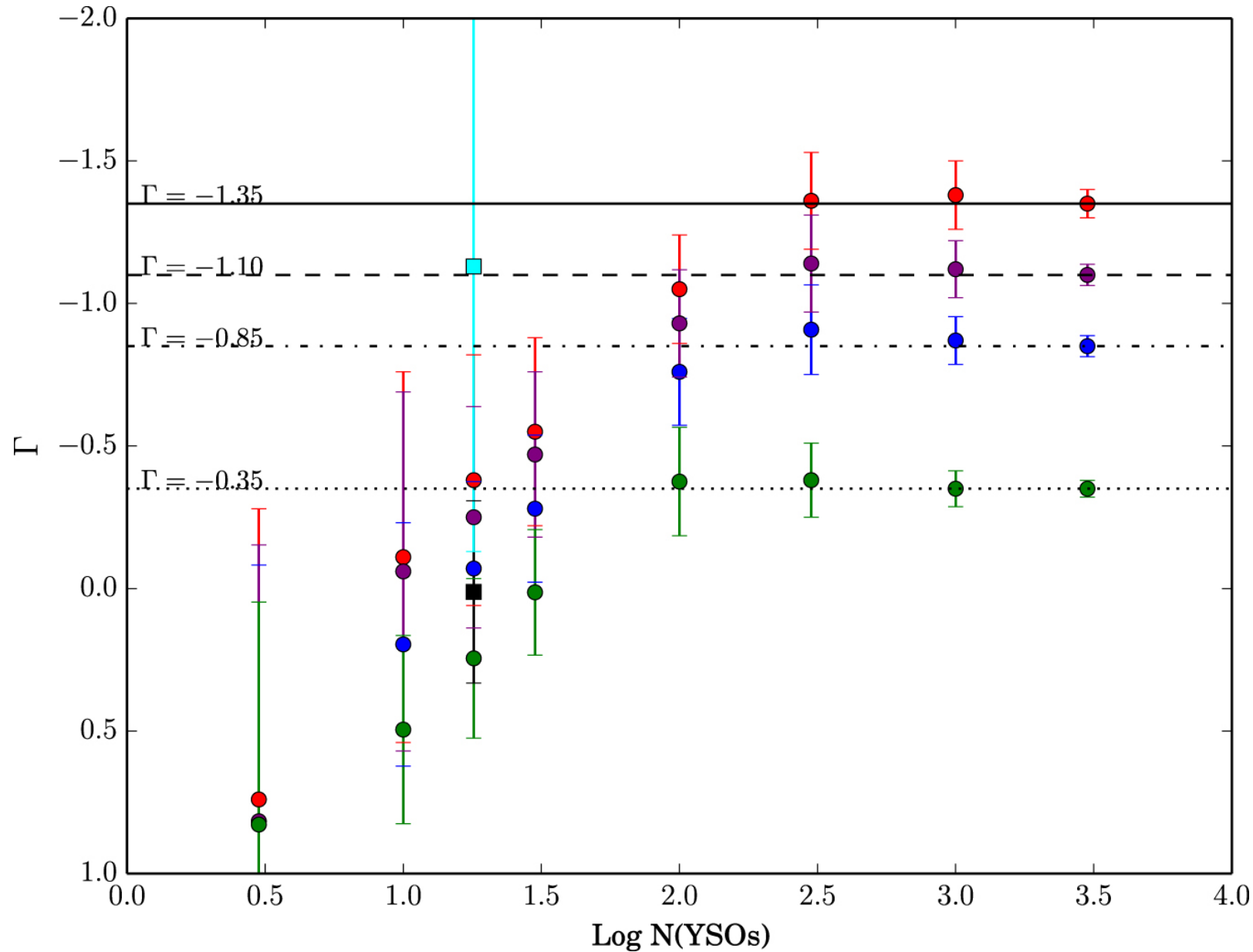
Figure 8. from High-resolution Observations of the Molecular Clouds Associated with the Huge H II Region CTB 102 null 2019 APJ 876 45 doi:10.3847/1538-4357/ab1264 https://dx.doi.org/10.3847/1538-4357/ab1264 © 2019. The American Astronomical Society. All rights reserved.
