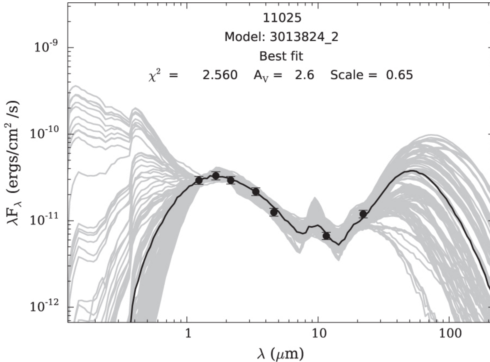
Figure 7. from High-resolution Observations of the Molecular Clouds Associated with the Huge H II Region CTB 102 null 2019 APJ 876 45 doi:10.3847/1538-4357/ab1264 https://dx.doi.org/10.3847/1538-4357/ab1264 © 2019. The American Astronomical Society. All rights reserved.
