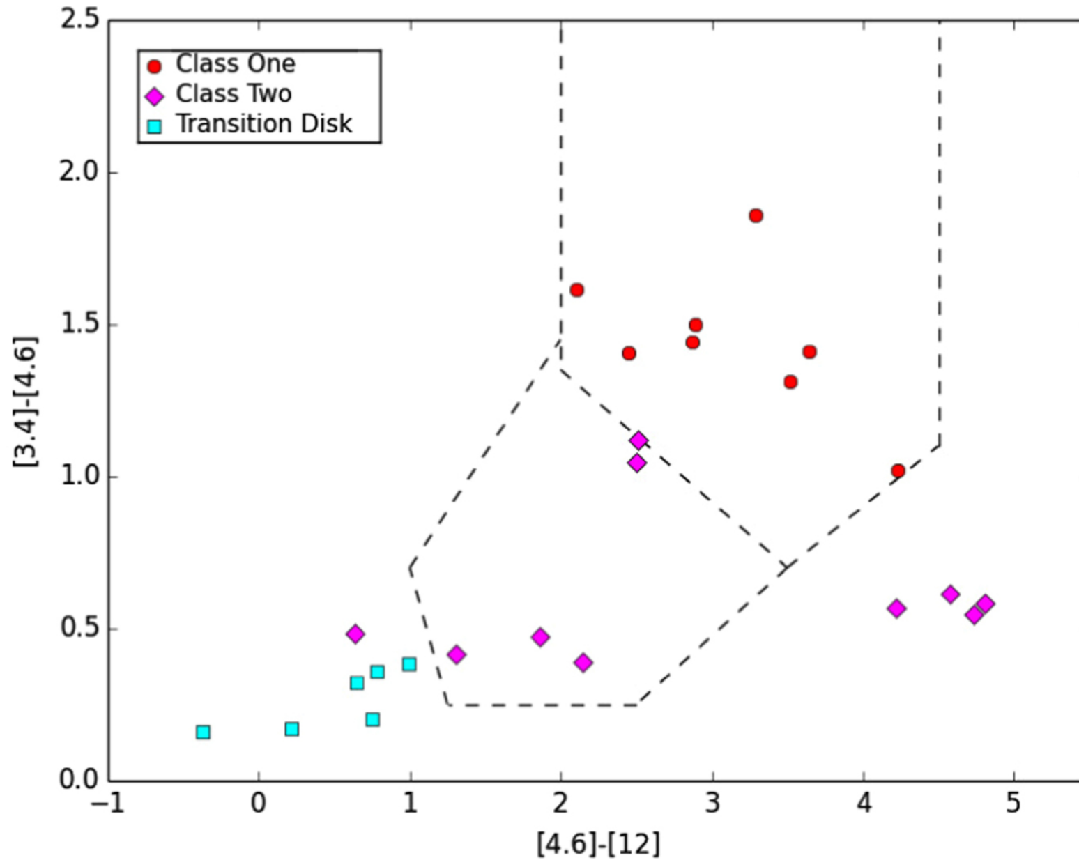
Figure 5. from High-resolution Observations of the Molecular Clouds Associated with the Huge H II Region CTB 102 null 2019 APJ 876 45 doi:10.3847/1538-4357/ab1264 https://dx.doi.org/10.3847/1538-4357/ab1264 © 2019. The American Astronomical Society. All rights reserved.
