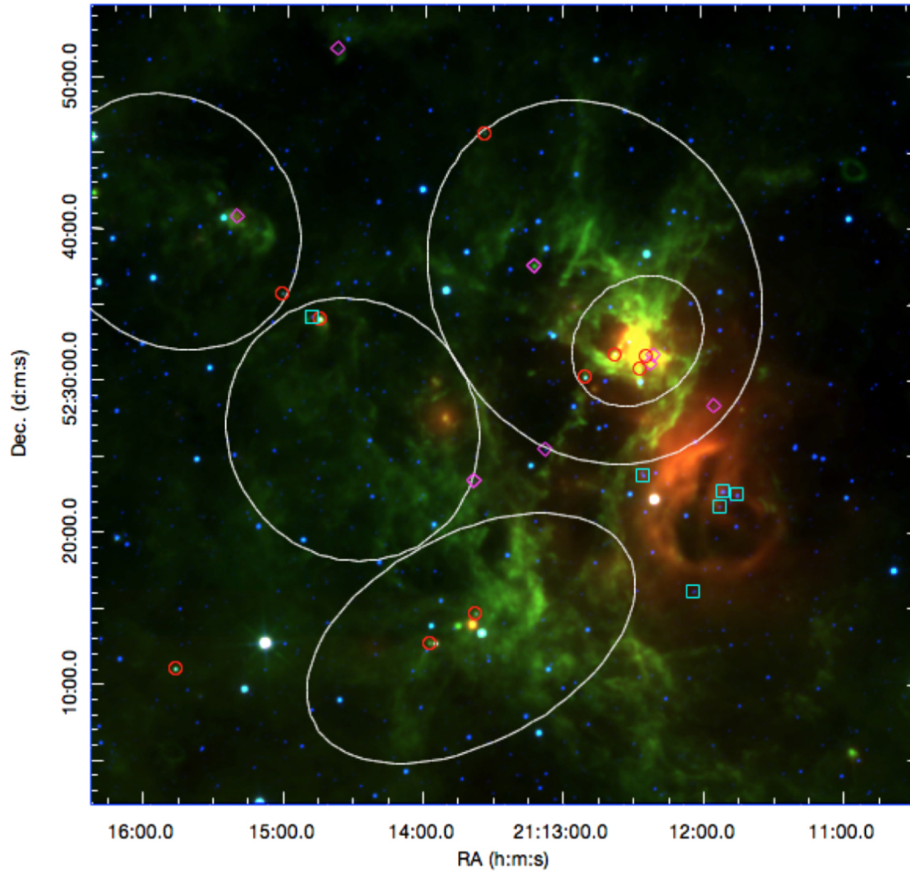
Figure 4. from High-resolution Observations of the Molecular Clouds Associated with the Huge H II Region CTB 102 null 2019 APJ 876 45 doi:10.3847/1538-4357/ab1264 https://dx.doi.org/10.3847/1538-4357/ab1264 © 2019. The American Astronomical Society. All rights reserved.
