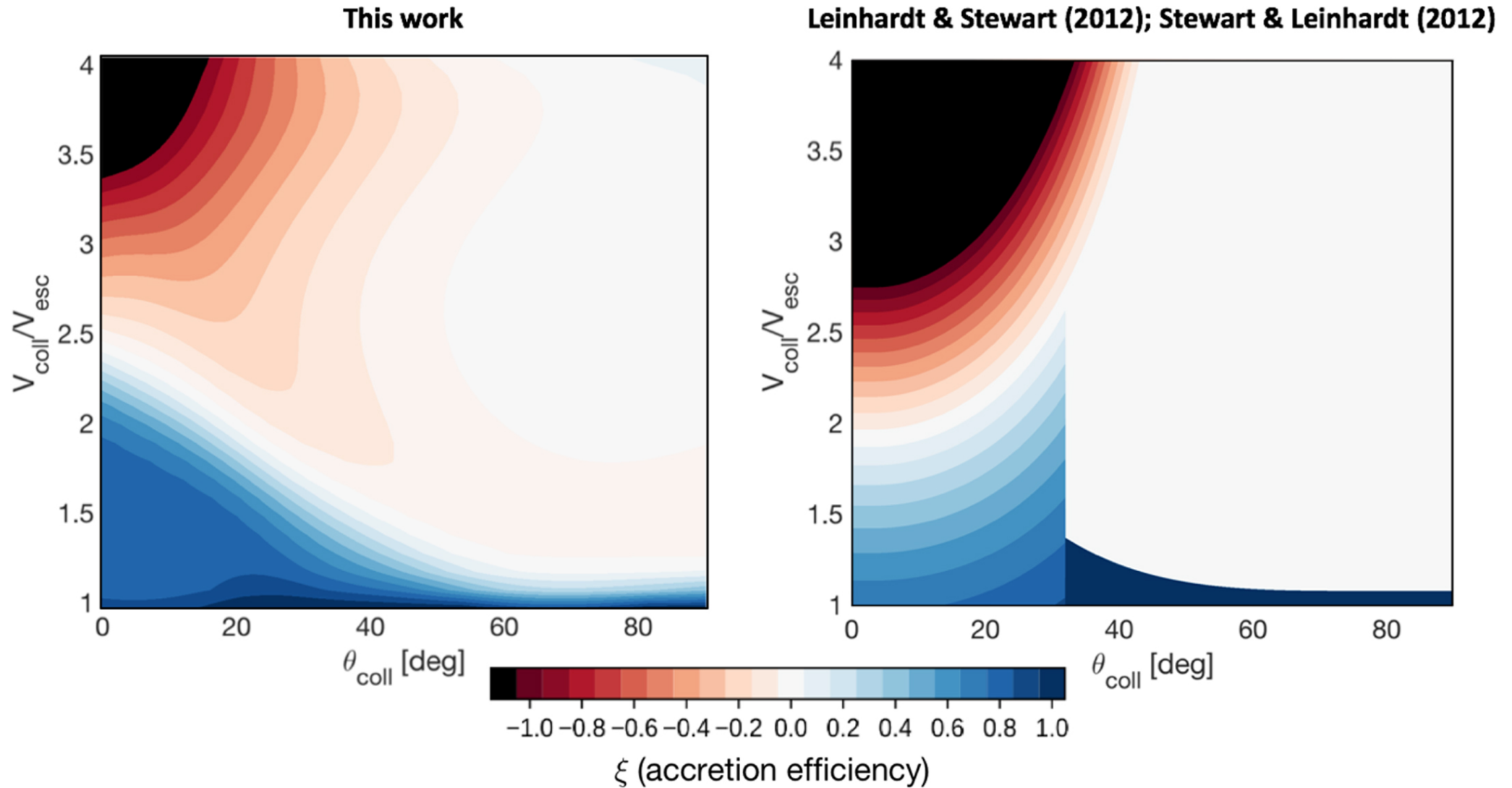
Figure 6. from Realistic On-the-fly Outcomes of Planetary Collisions: Machine Learning Applied to Simulations of Giant Impacts null 2019 APJ 875 40 doi:10.3847/1538-4357/ab0e8a https://dx.doi.org/10.3847/1538-4357/ab0e8a © 2019. The American Astronomical Society. All rights reserved.
