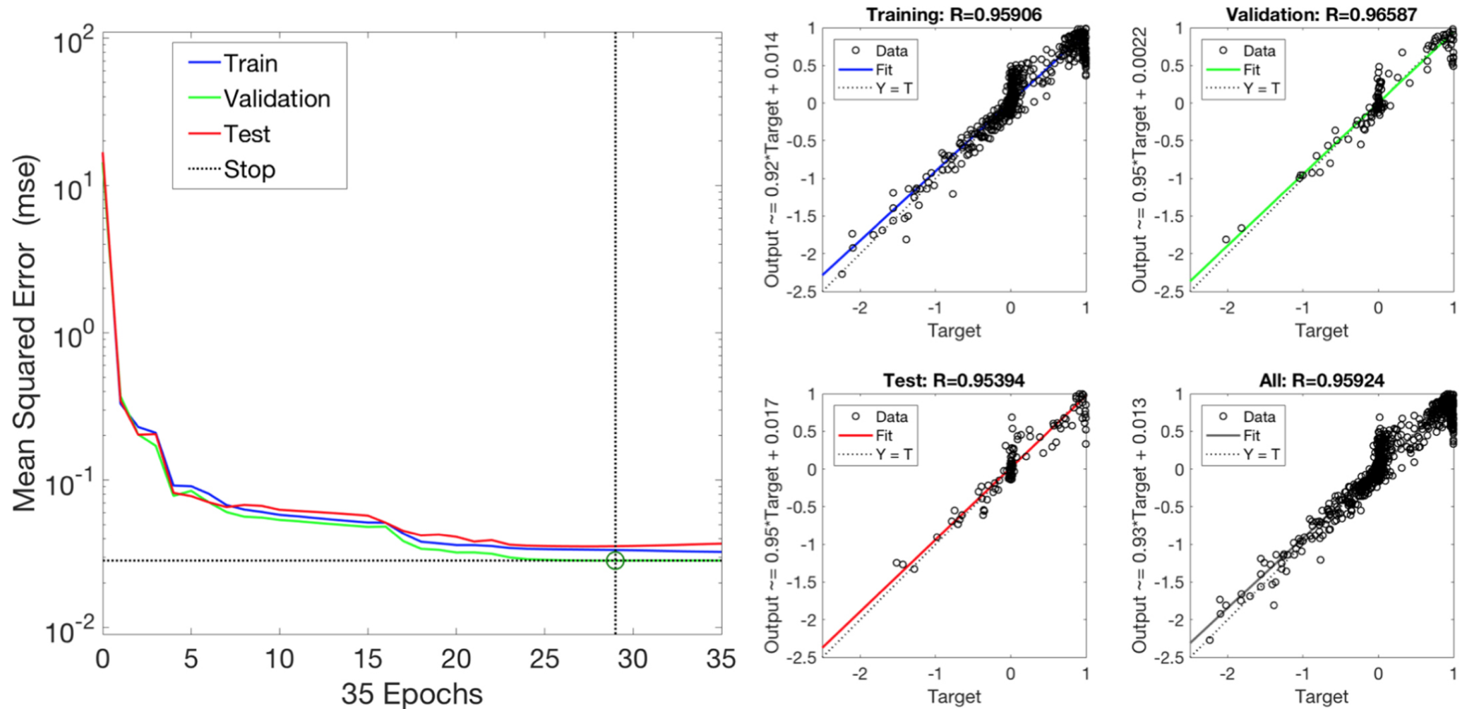
Figure 5. from Realistic On-the-fly Outcomes of Planetary Collisions: Machine Learning Applied to Simulations of Giant Impacts null 2019 APJ 875 40 doi:10.3847/1538-4357/ab0e8a https://dx.doi.org/10.3847/1538-4357/ab0e8a © 2019. The American Astronomical Society. All rights reserved.
