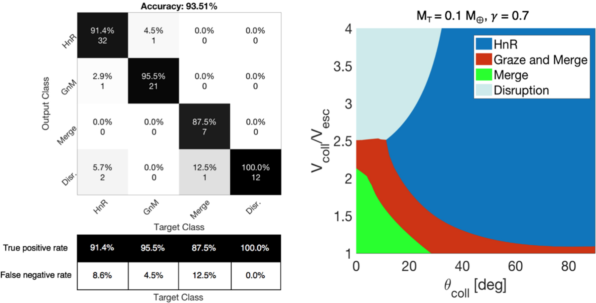
Figure 4. from Realistic On-the-fly Outcomes of Planetary Collisions: Machine Learning Applied to Simulations of Giant Impacts null 2019 APJ 875 40 doi:10.3847/1538-4357/ab0e8a https://dx.doi.org/10.3847/1538-4357/ab0e8a © 2019. The American Astronomical Society. All rights reserved.
