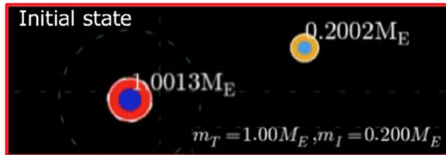
Figure 2. from Realistic On-the-fly Outcomes of Planetary Collisions: Machine Learning Applied to Simulations of Giant Impacts null 2019 APJ 875 40 doi:10.3847/1538-4357/ab0e8a https://dx.doi.org/10.3847/1538-4357/ab0e8a © 2019. The American Astronomical Society. All rights reserved.
