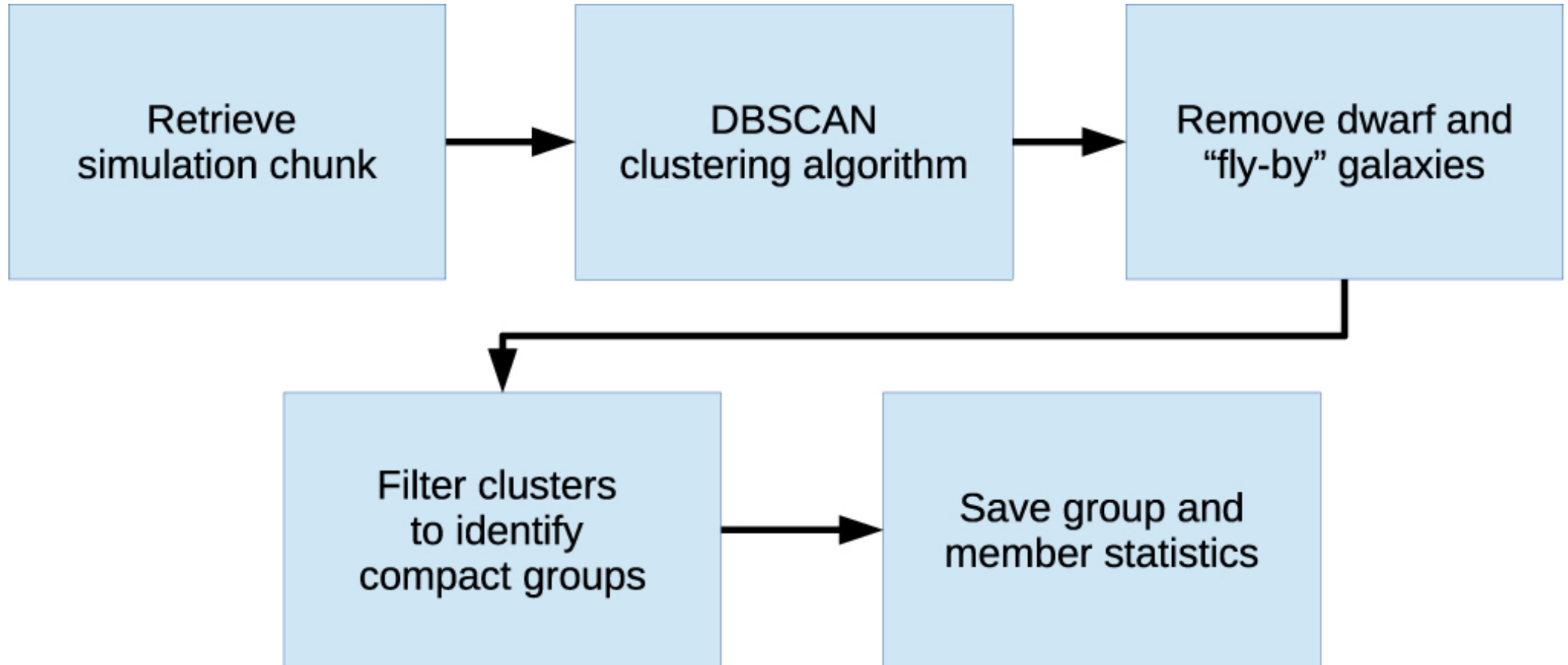
Figure 1. from The Occurrence of Compact Groups of Galaxies through Cosmic Time null 2019 APJ 873 124 doi:10.3847/1538-4357/ab053e https://dx.doi.org/10.3847/1538-4357/ab053e © 2019. The American Astronomical Society. All rights reserved.
