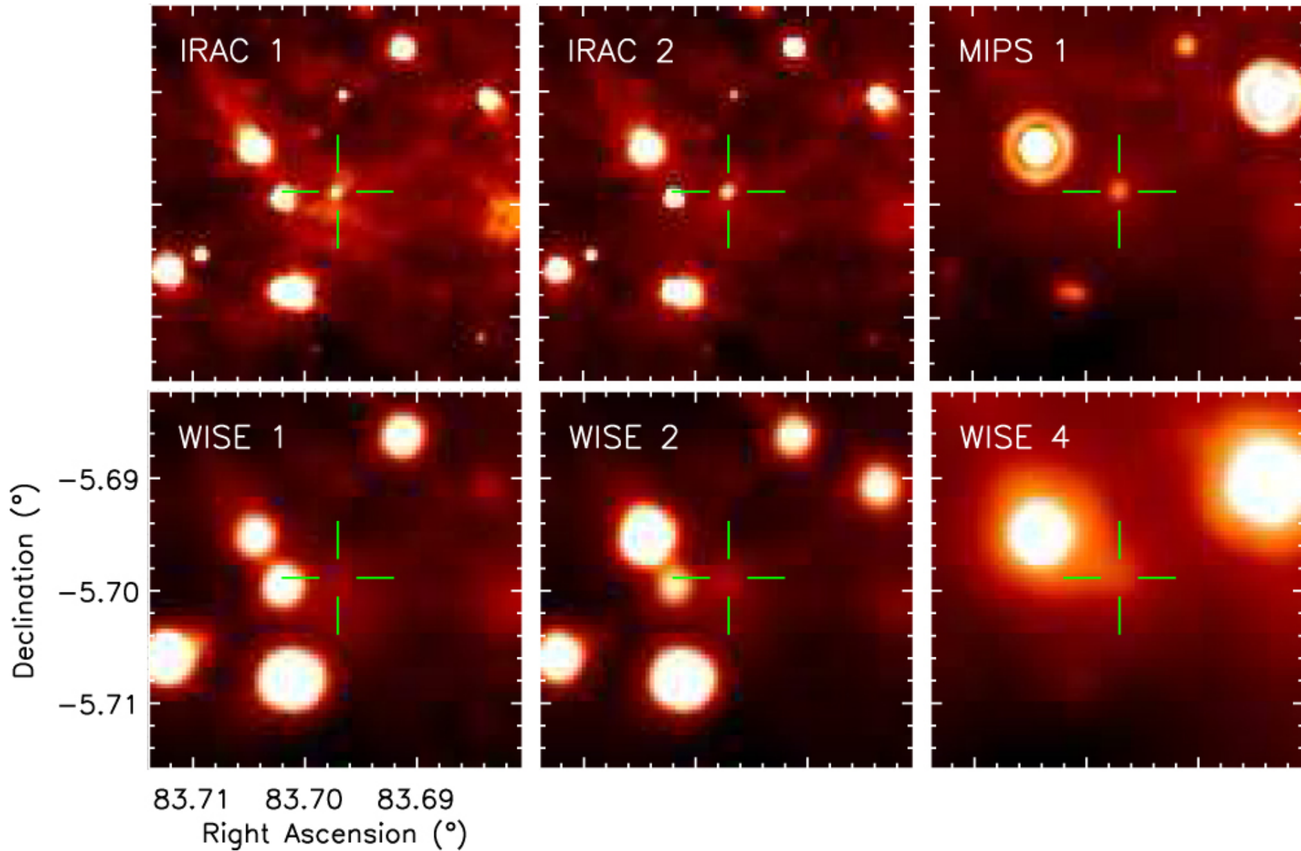
Figure 8. from Constraining the Rate of Protostellar Accretion Outbursts in the Orion Molecular Clouds null 2019 APJ 872 183 doi:10.3847/1538-4357/ab01dc https://dx.doi.org/10.3847/1538-4357/ab01dc © 2019. The American Astronomical Society. All rights reserved.
