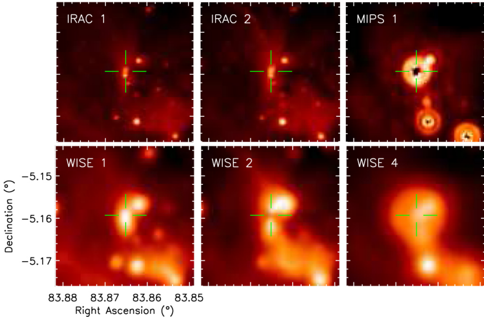
Figure 7. from Constraining the Rate of Protostellar Accretion Outbursts in the Orion Molecular Clouds null 2019 APJ 872 183 doi:10.3847/1538-4357/ab01dc https://dx.doi.org/10.3847/1538-4357/ab01dc © 2019. The American Astronomical Society. All rights reserved.
