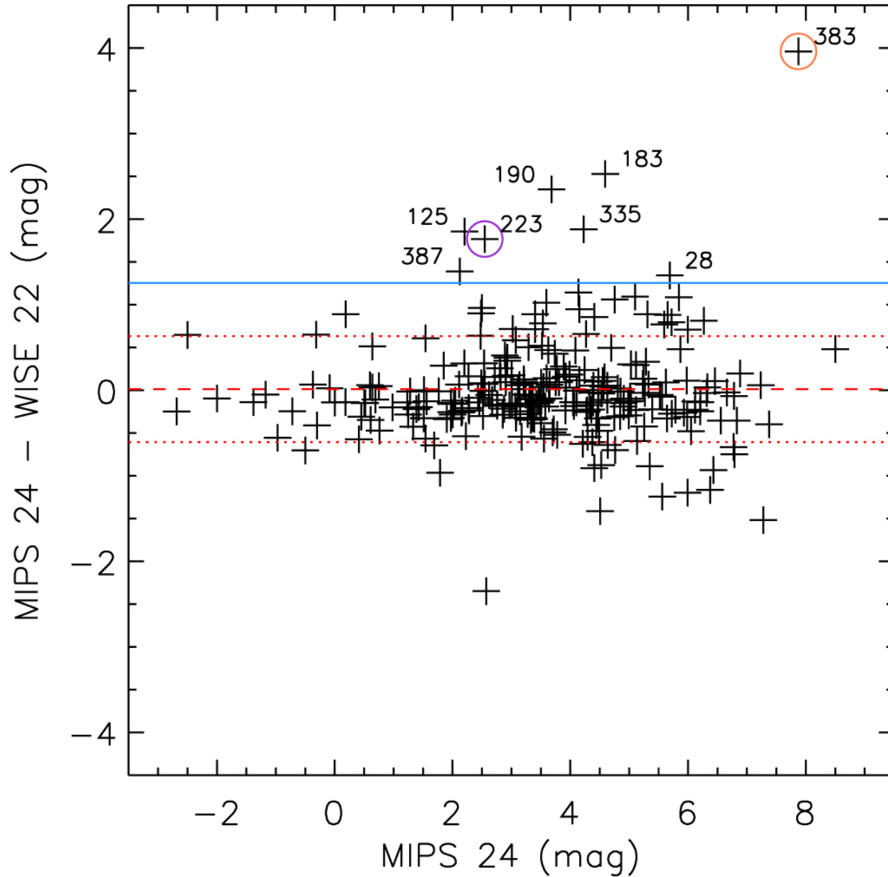
Figure 3. from Constraining the Rate of Protostellar Accretion Outbursts in the Orion Molecular Clouds null 2019 APJ 872 183 doi:10.3847/1538-4357/ab01dc https://dx.doi.org/10.3847/1538-4357/ab01dc © 2019. The American Astronomical Society. All rights reserved.
