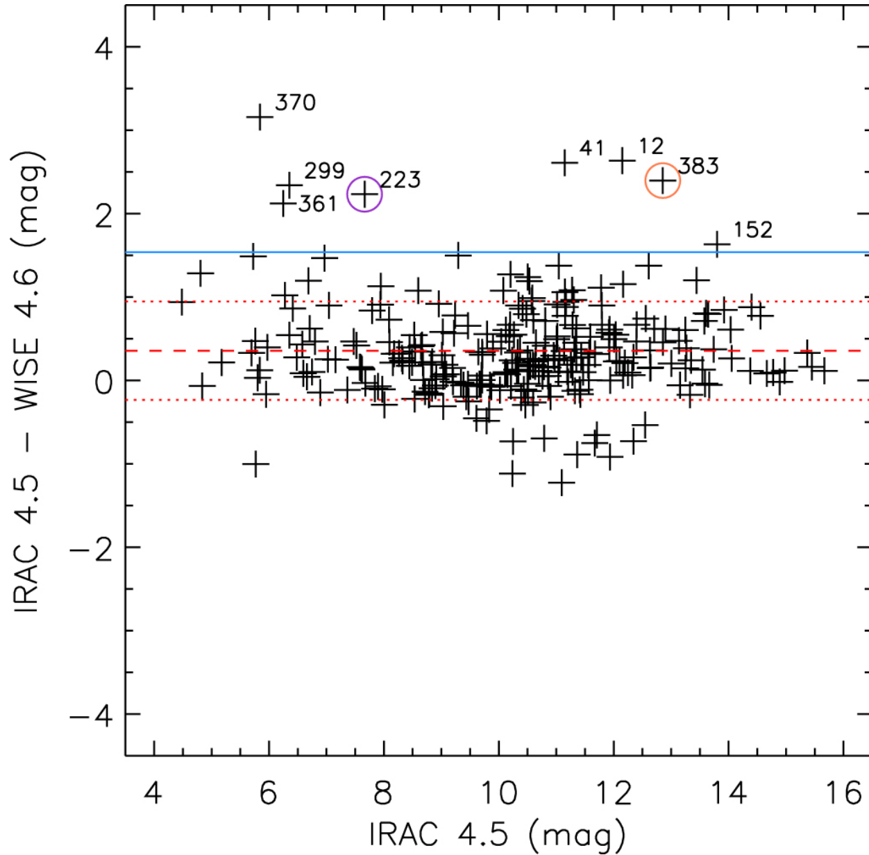
Figure 2. from Constraining the Rate of Protostellar Accretion Outbursts in the Orion Molecular Clouds null 2019 APJ 872 183 doi:10.3847/1538-4357/ab01dc https://dx.doi.org/10.3847/1538-4357/ab01dc © 2019. The American Astronomical Society. All rights reserved.
