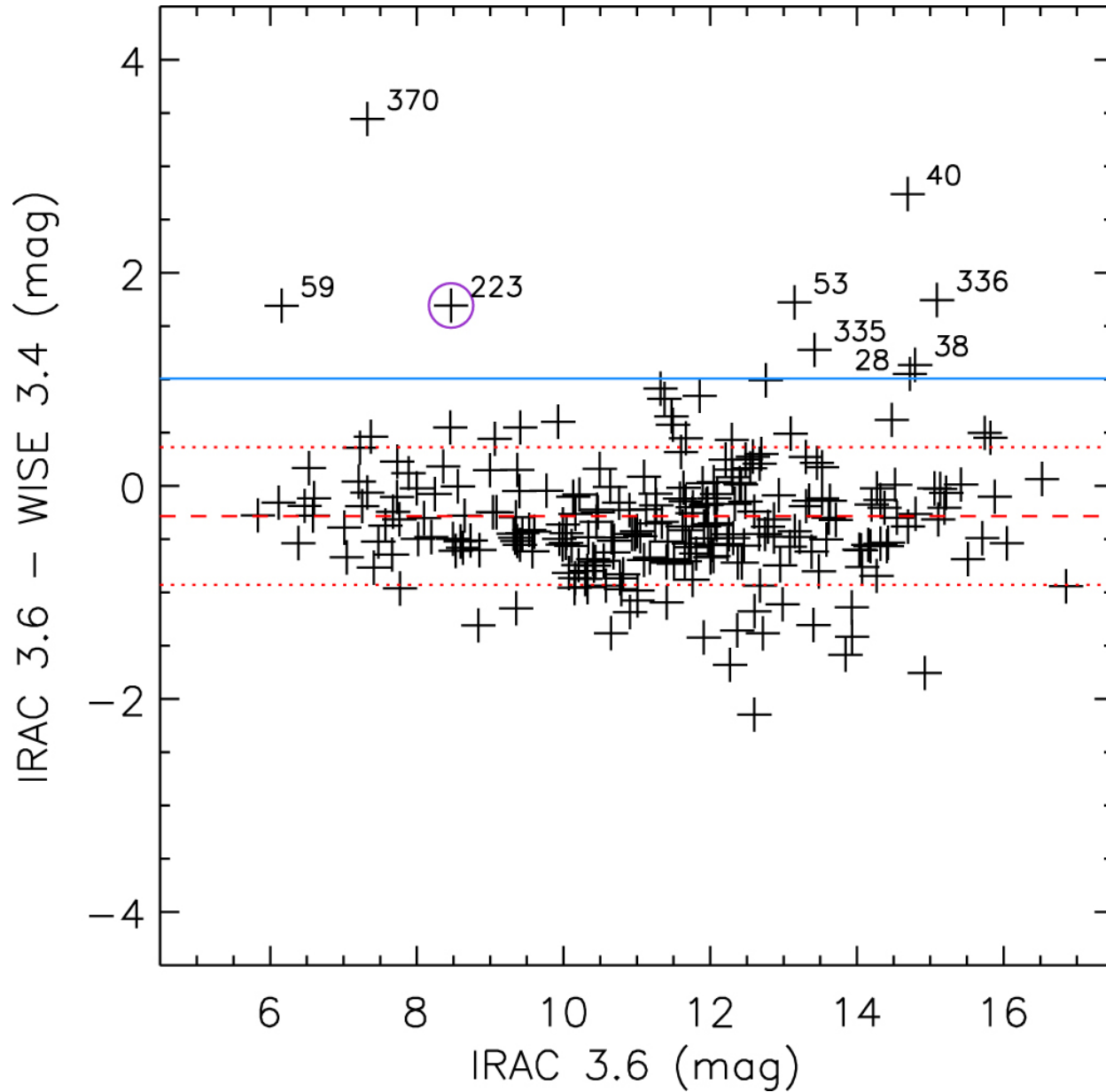
Figure 1. from Constraining the Rate of Protostellar Accretion Outbursts in the Orion Molecular Clouds null 2019 APJ 872 183 doi:10.3847/1538-4357/ab01dc https://dx.doi.org/10.3847/1538-4357/ab01dc © 2019. The American Astronomical Society. All rights reserved.
