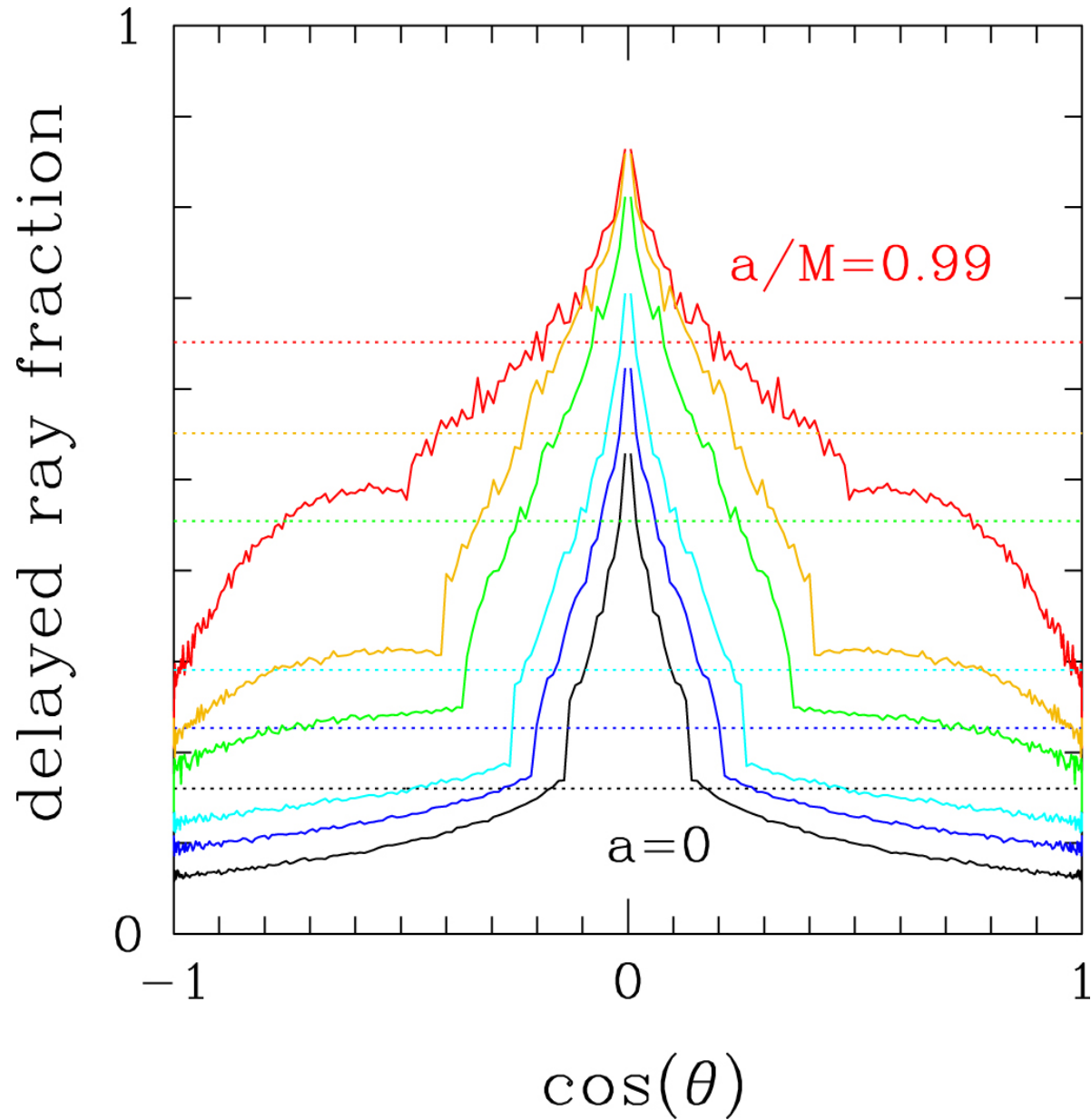
Figure 9. from Impulsive Electromagnetic Emission near a Black Hole null 2019 APJ 874 48 doi:10.3847/1538-4357/aafda3 https://dx.doi.org/10.3847/1538-4357/aafda3 © 2019. The American Astronomical Society. All rights reserved.
