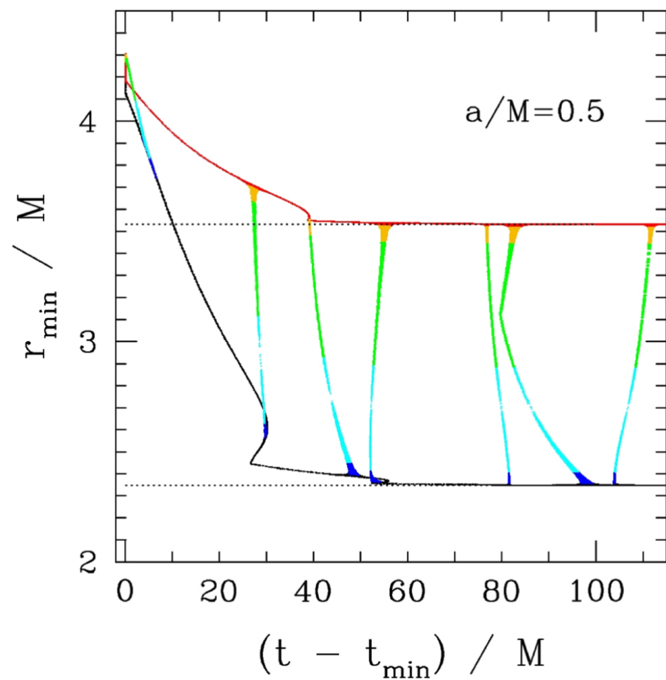
Figure 8. from Impulsive Electromagnetic Emission near a Black Hole null 2019 APJ 874 48 doi:10.3847/1538-4357/aafda3 https://dx.doi.org/10.3847/1538-4357/aafda3 © 2019. The American Astronomical Society. All rights reserved.
