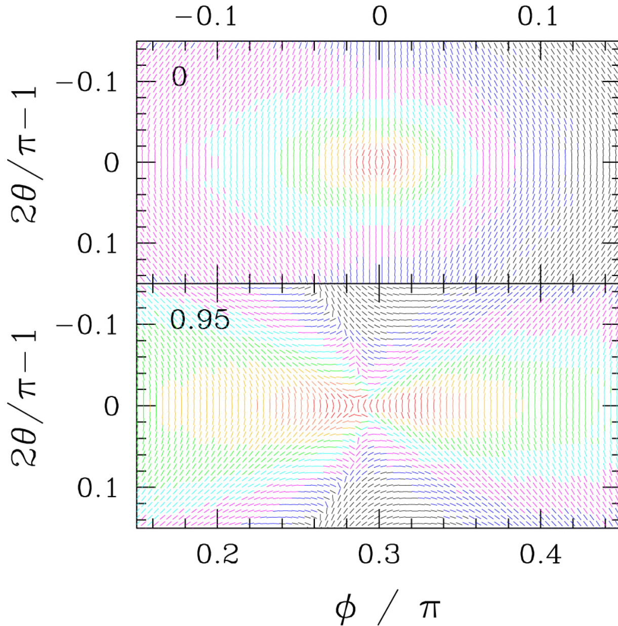
Figure 6. from Impulsive Electromagnetic Emission near a Black Hole null 2019 APJ 874 48 doi:10.3847/1538-4357/aafda3 https://dx.doi.org/10.3847/1538-4357/aafda3 © 2019. The American Astronomical Society. All rights reserved.
