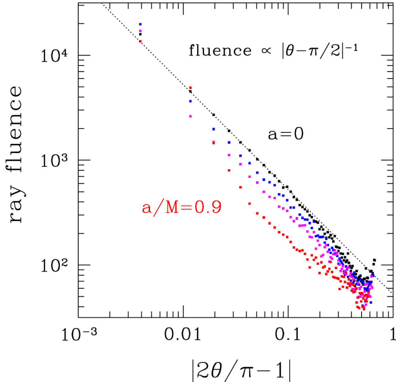
Figure 3. from Impulsive Electromagnetic Emission near a Black Hole null 2019 APJ 874 48 doi:10.3847/1538-4357/aafda3 https://dx.doi.org/10.3847/1538-4357/aafda3 © 2019. The American Astronomical Society. All rights reserved.
