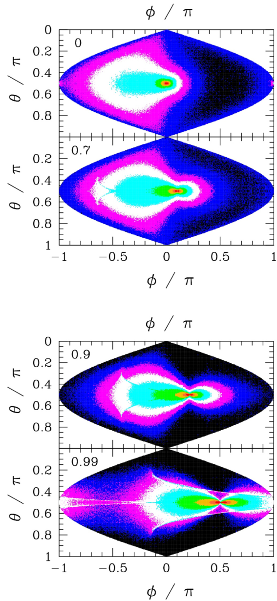
Figure 2. from Impulsive Electromagnetic Emission near a Black Hole null 2019 APJ 874 48 doi:10.3847/1538-4357/aafda3 https://dx.doi.org/10.3847/1538-4357/aafda3 © 2019. The American Astronomical Society. All rights reserved.
