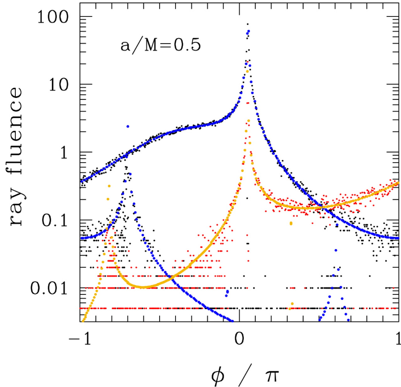
Figure 17. from Impulsive Electromagnetic Emission near a Black Hole null 2019 APJ 874 48 doi:10.3847/1538-4357/aafda3 https://dx.doi.org/10.3847/1538-4357/aafda3 © 2019. The American Astronomical Society. All rights reserved.
