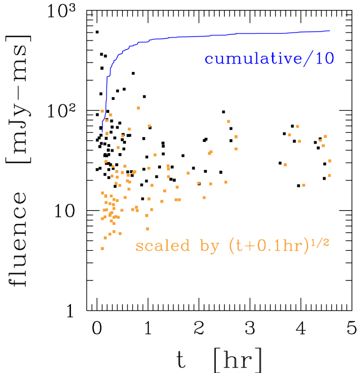
Figure 16. from Impulsive Electromagnetic Emission near a Black Hole null 2019 APJ 874 48 doi:10.3847/1538-4357/aafda3 https://dx.doi.org/10.3847/1538-4357/aafda3 © 2019. The American Astronomical Society. All rights reserved.
