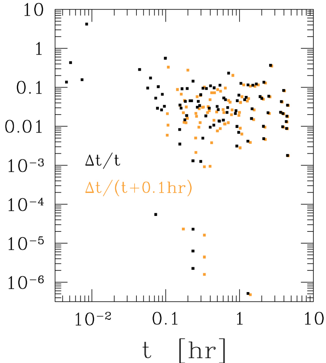
Figure 15. from Impulsive Electromagnetic Emission near a Black Hole null 2019 APJ 874 48 doi:10.3847/1538-4357/aafda3 https://dx.doi.org/10.3847/1538-4357/aafda3 © 2019. The American Astronomical Society. All rights reserved.
