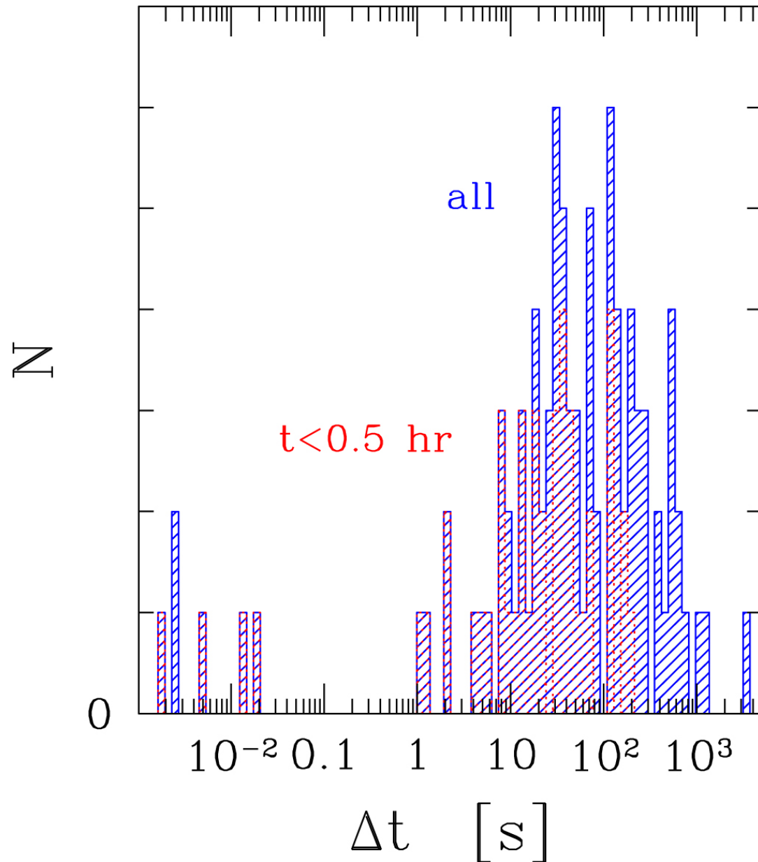
Figure 14. from Impulsive Electromagnetic Emission near a Black Hole null 2019 APJ 874 48 doi:10.3847/1538-4357/aafda3 https://dx.doi.org/10.3847/1538-4357/aafda3 © 2019. The American Astronomical Society. All rights reserved.
