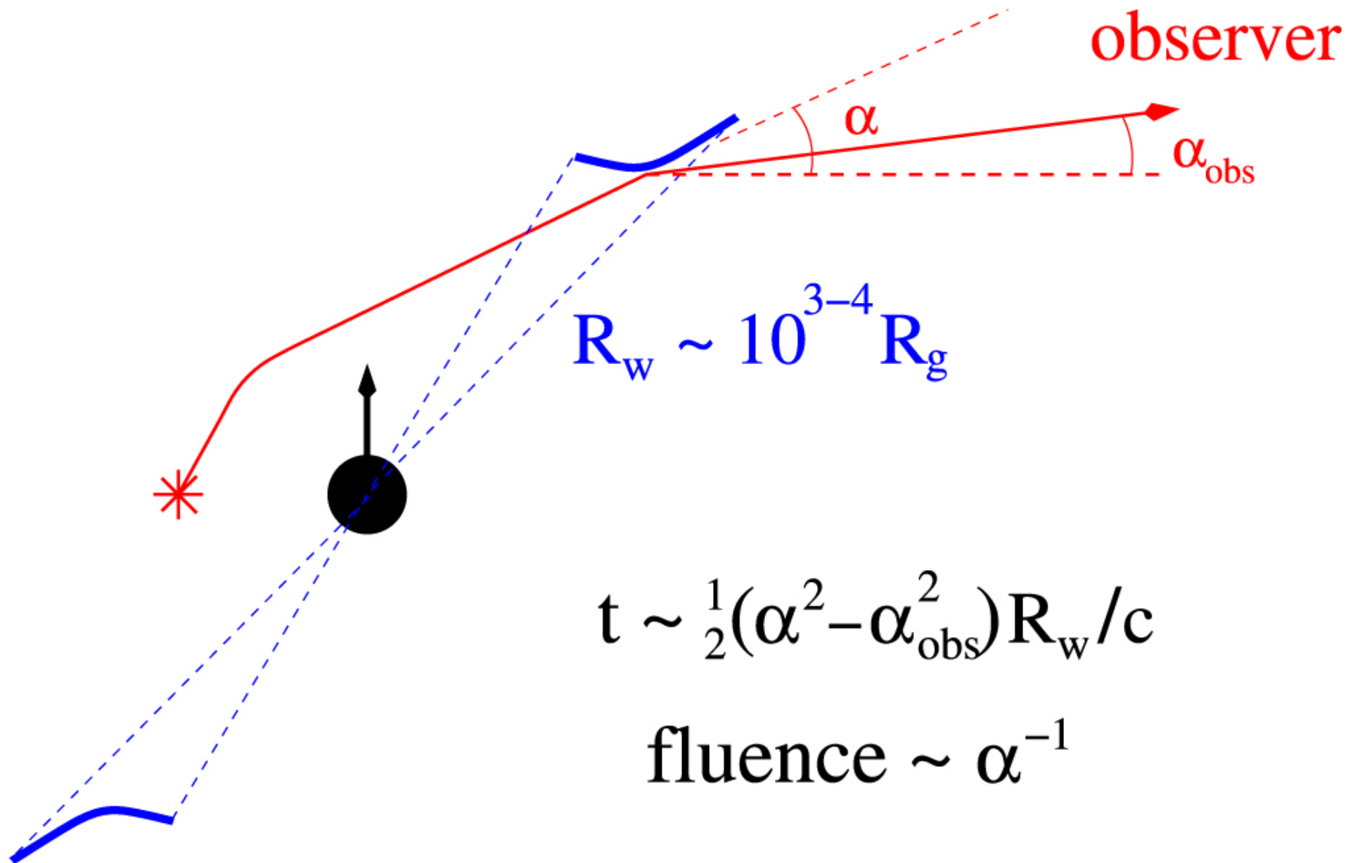
Figure 13. from Impulsive Electromagnetic Emission near a Black Hole null 2019 APJ 874 48 doi:10.3847/1538-4357/aafda3 https://dx.doi.org/10.3847/1538-4357/aafda3 © 2019. The American Astronomical Society. All rights reserved.
