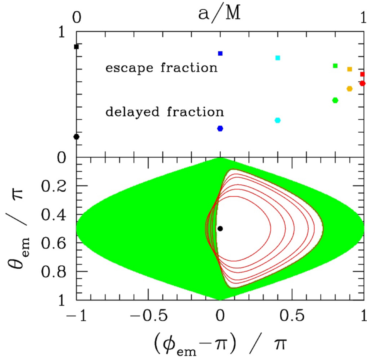
Figure 1. from Impulsive Electromagnetic Emission near a Black Hole null 2019 APJ 874 48 doi:10.3847/1538-4357/aafda3 https://dx.doi.org/10.3847/1538-4357/aafda3 © 2019. The American Astronomical Society. All rights reserved.
