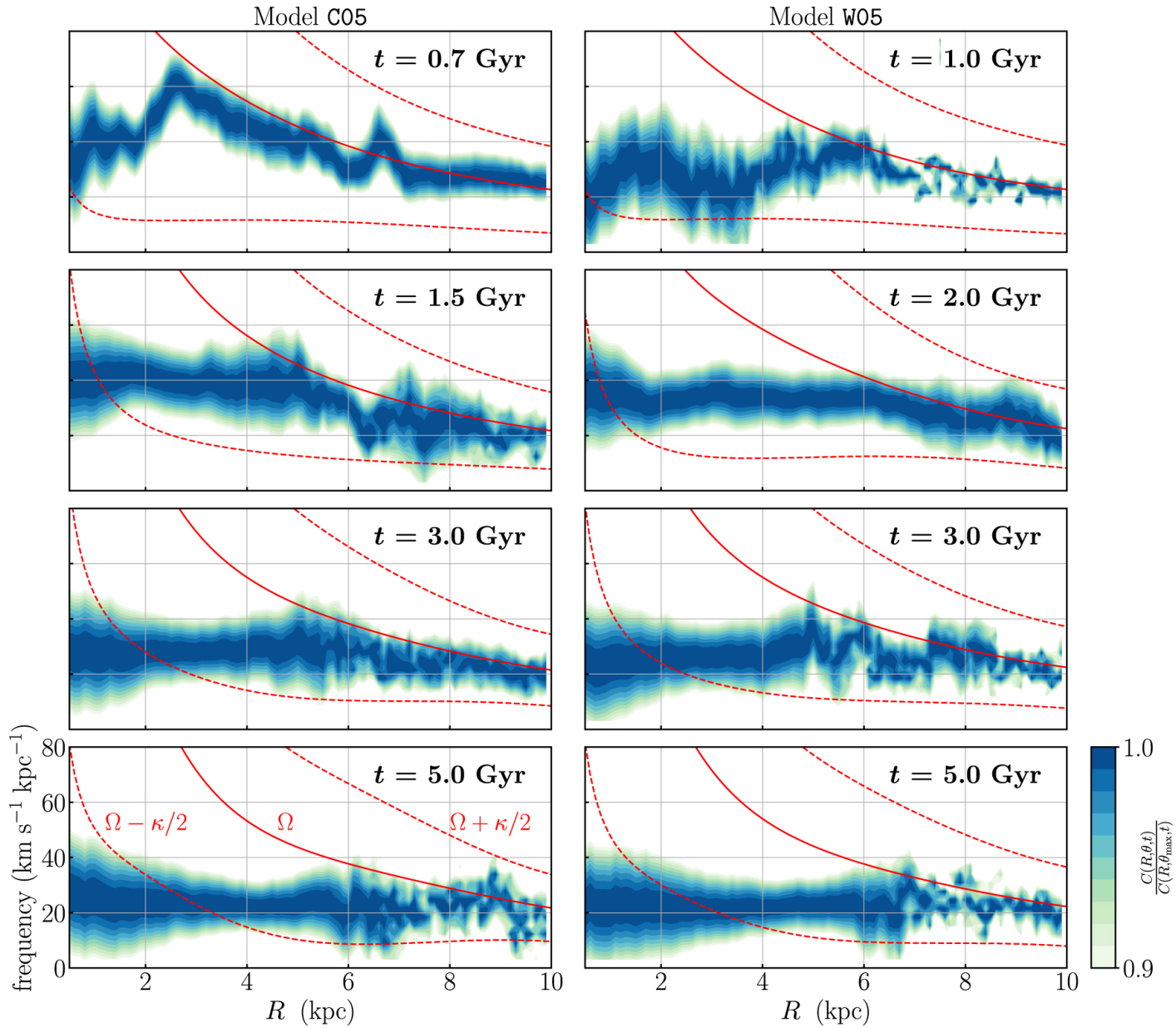
Figure 8. from Effects of Gas on Formation and Evolution of Stellar Bars and Nuclear Rings in Disk Galaxies null 2019 APJ 872 5 doi:10.3847/1538-4357/aafc5f https://dx.doi.org/10.3847/1538-4357/aafc5f © 2019. The American Astronomical Society. All rights reserved.
