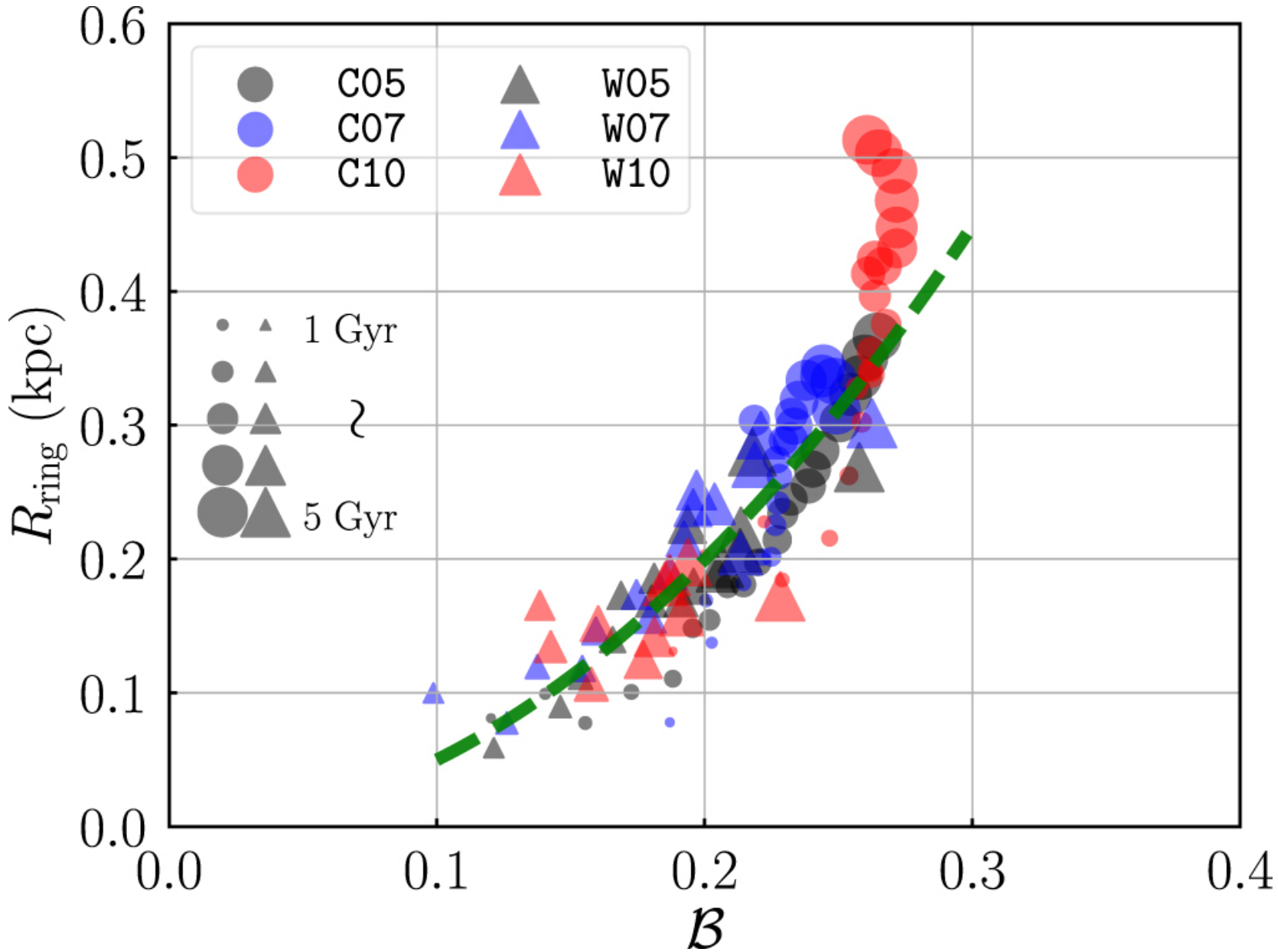
Figure 21. from Effects of Gas on Formation and Evolution of Stellar Bars and Nuclear Rings in Disk Galaxies null 2019 APJ 872 5 doi:10.3847/1538-4357/aafc5f https://dx.doi.org/10.3847/1538-4357/aafc5f © 2019. The American Astronomical Society. All rights reserved.
