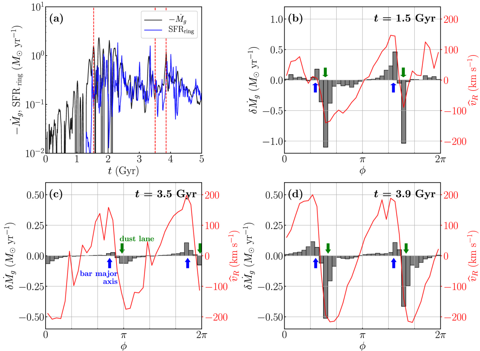
Figure 16. from Effects of Gas on Formation and Evolution of Stellar Bars and Nuclear Rings in Disk Galaxies null 2019 APJ 872 5 doi:10.3847/1538-4357/aafc5f https://dx.doi.org/10.3847/1538-4357/aafc5f © 2019. The American Astronomical Society. All rights reserved.
