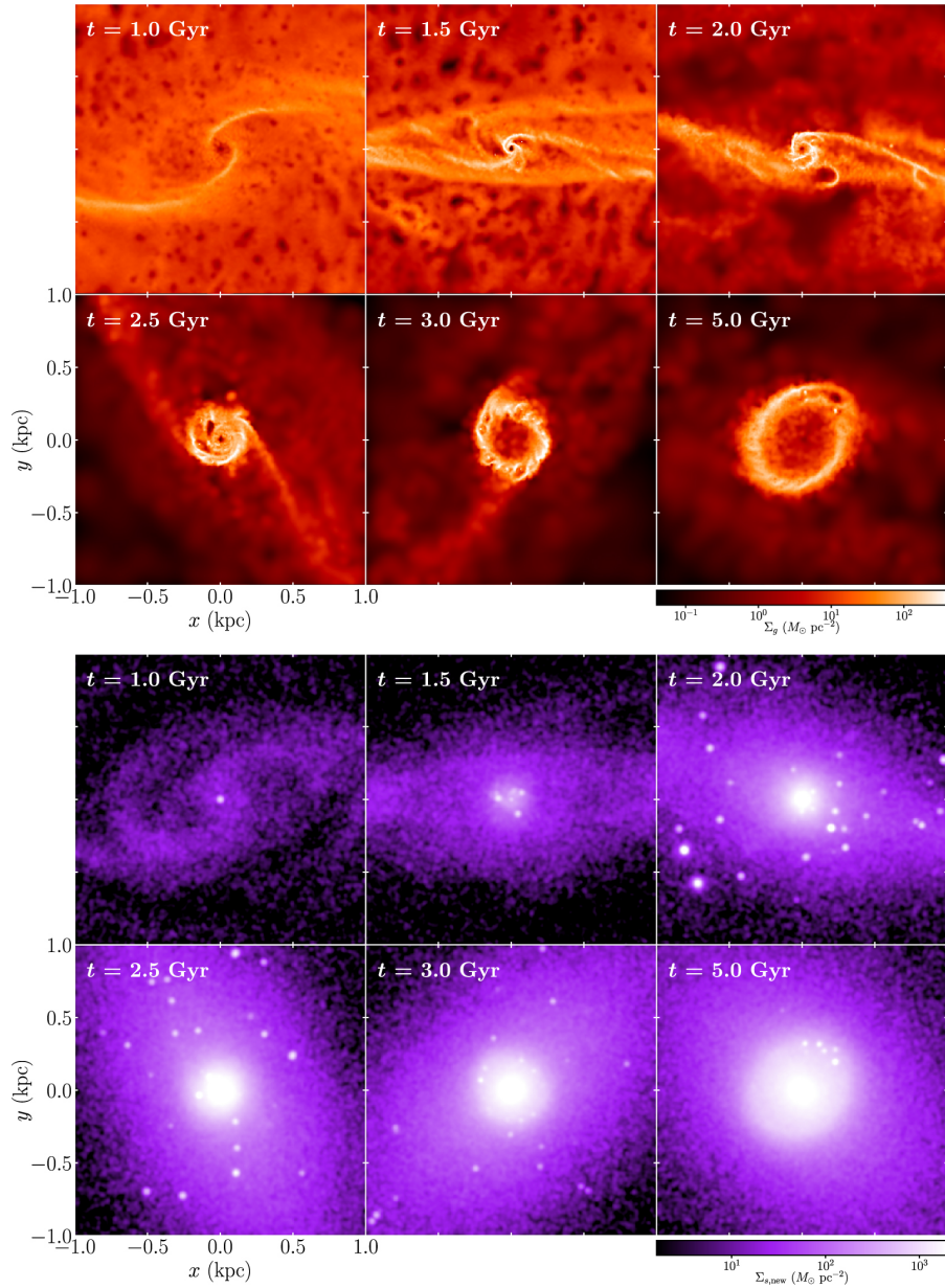
Figure 15. from Effects of Gas on Formation and Evolution of Stellar Bars and Nuclear Rings in Disk Galaxies null 2019 APJ 872 5 doi:10.3847/1538-4357/aafc5f https://dx.doi.org/10.3847/1538-4357/aafc5f © 2019. The American Astronomical Society. All rights reserved.
