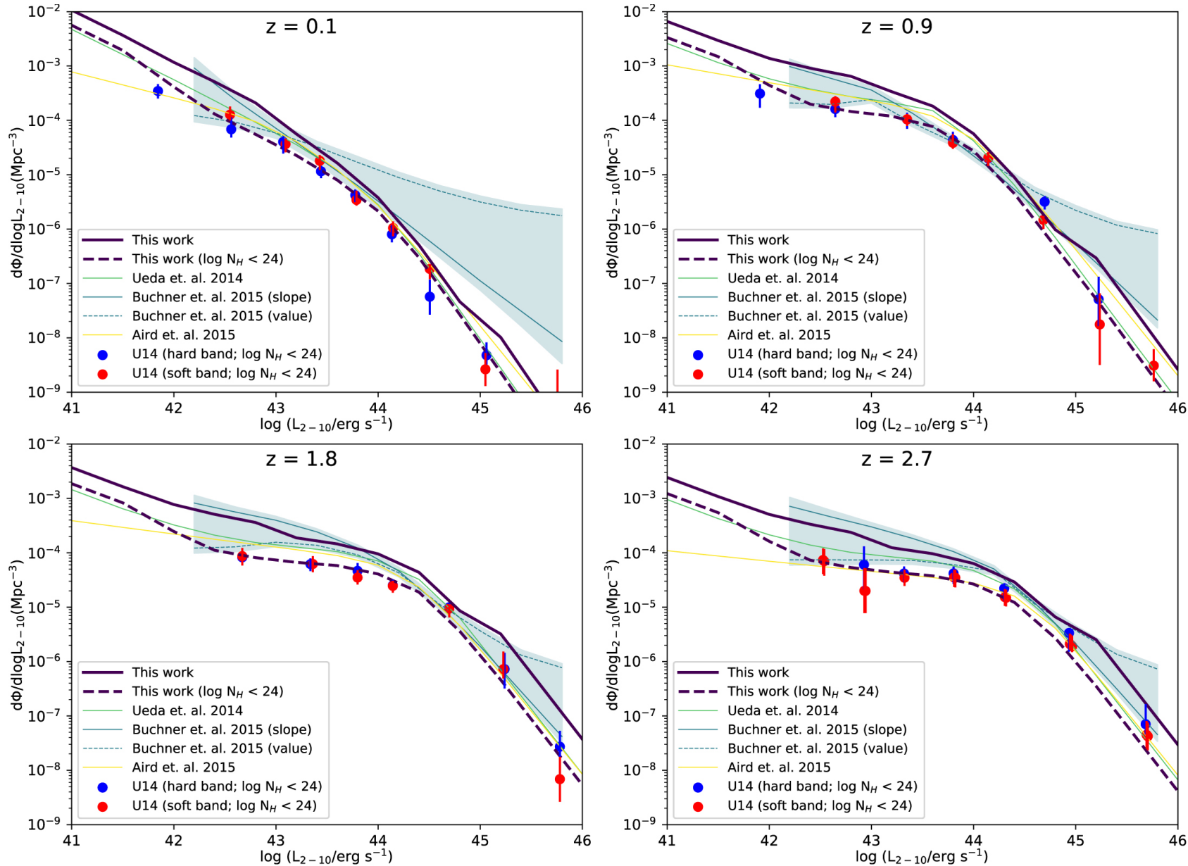
Figure 9. from The Accretion History of AGNs. I. Supermassive Black Hole Population Synthesis Model null 2019 APJ 871 240 doi:10.3847/1538-4357/aafb77 https://dx.doi.org/10.3847/1538-4357/aafb77
