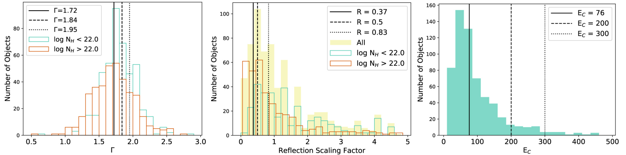
Figure 5. from The Accretion History of AGNs. I. Supermassive Black Hole Population Synthesis Model null 2019 APJ 871 240 doi:10.3847/1538-4357/aafb77 https://dx.doi.org/10.3847/1538-4357/aafb77 © 2019. The American Astronomical Society. All rights reserved.
