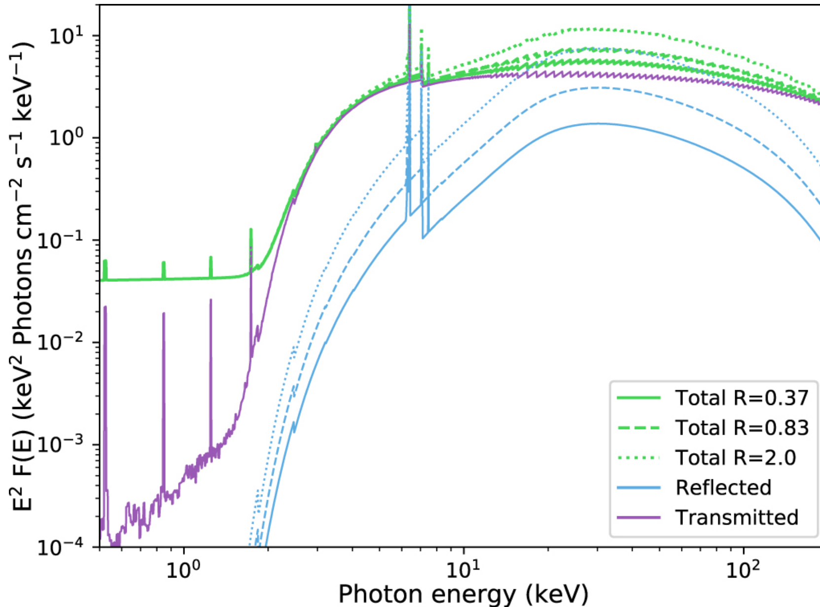
Figure 4. from The Accretion History of AGNs. I. Supermassive Black Hole Population Synthesis Model null 2019 APJ 871 240 doi:10.3847/1538-4357/aafb77 https://dx.doi.org/10.3847/1538-4357/aafb77 © 2019. The American Astronomical Society. All rights reserved.
