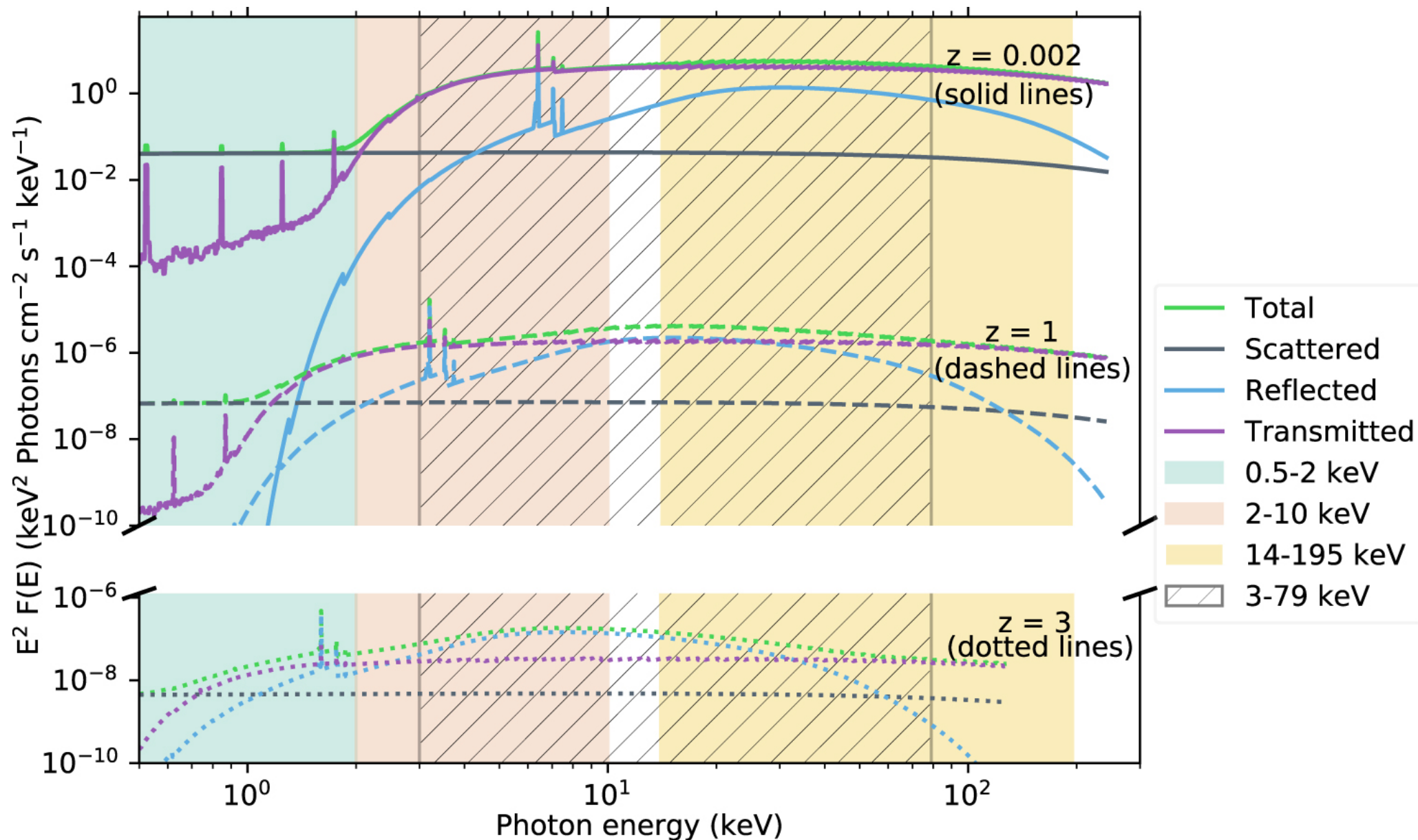
Figure 1. from The Accretion History of AGNs. I. Supermassive Black Hole Population Synthesis Model null 2019 APJ 871 240 doi:10.3847/1538-4357/aafb77 https://dx.doi.org/10.3847/1538-4357/aafb77 © 2019. The American Astronomical Society. All rights reserved.
