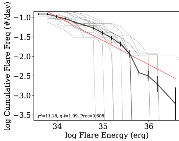
Figure 9. from The Evolution of Flare Activity with Stellar Age null 2019 APJ 871 241 doi:10.3847/1538-4357/aafb76 https://dx.doi.org/10.3847/1538-4357/aafb76 © 2019. The American Astronomical Society.
